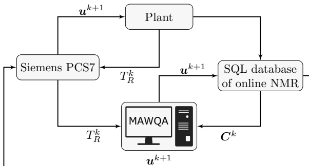
Fig. 2. Illustration of the setup used to communicate with the plant via the Siemens PCS7 system and via the SQL database of the online NMR.
