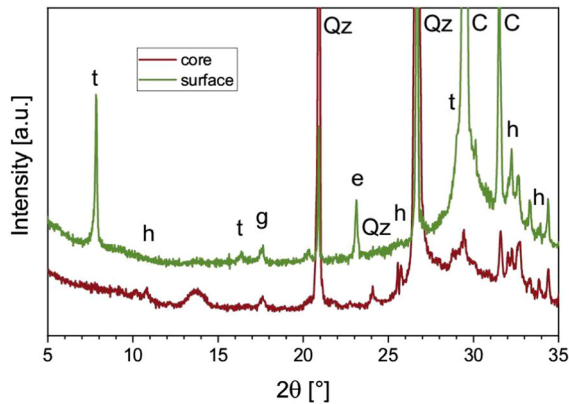
Fig. 9 X-ray diffractograms of hydrothermally treated UHPC samples (185 °C/1.1 MPa) with and without surface layer. t tobermorite, e ettringite, C clinker, h hydroxyllestadite, g hydrogarnet, Qz quartz
