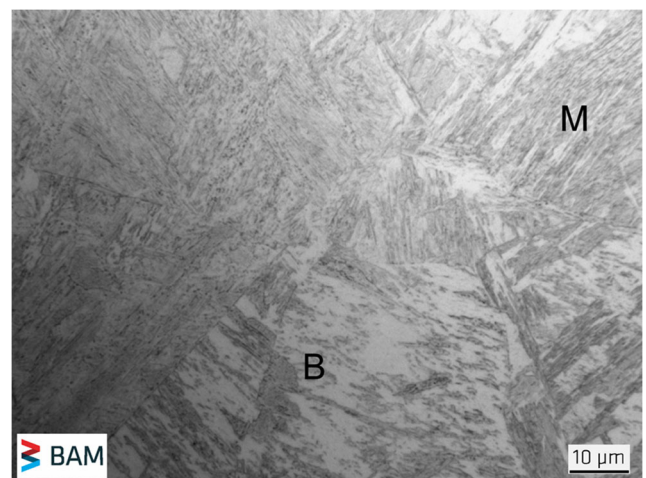
Fig. 10 Microstructure in the CGHAZ at t_{8/5} = 7 s
