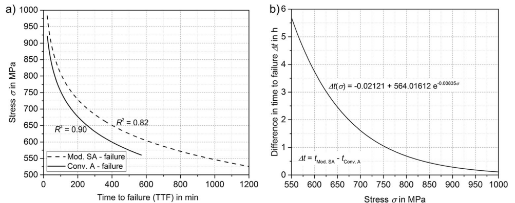
Fig. 14 (a) Regression functions of the implant stress vs. TTF (from Fig. 7) without measurement points; (b) corresponding TTF difference vs. applied implant stress
