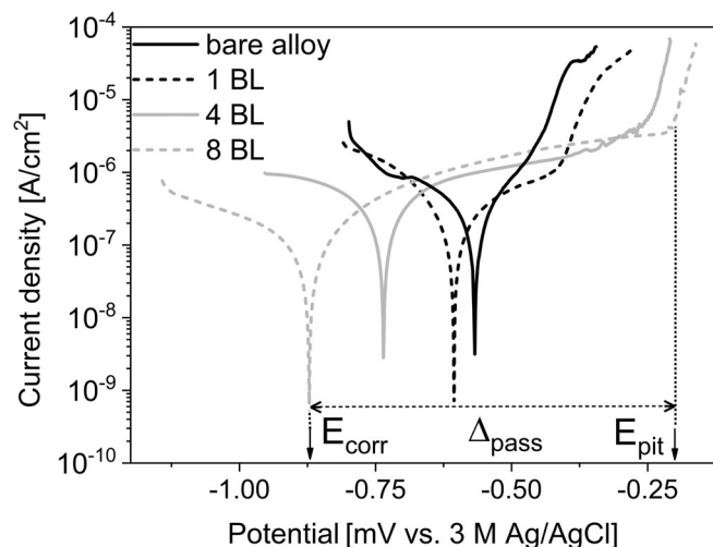
FIGURE 6 Tafel plots recorded in a 0.1 M NaClO 4 electrolyte solution at a scan rate of 1 mV s -1 on AA, (CNER/PEI) 1 /AA, (CNER/PEI) 4 /AA, and (CNER/PEI) 8 /AA. The corrosion E_{\text{corr}} and pitting E_{\text{pit}} potential are indicated in the graph for the 8BL system as an example. CNER, poly([o-cresyl glycidyl ether]-co-formaldehyde); PEI, poly-(ethylenimine)
