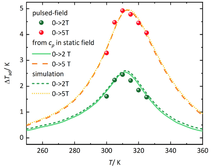
Fig. 2. Comparison of the adiabatic temperature change \Delta T_{ad} of the separated \text{La}(\text{Fe,Co,Si})_{13} -core determined indirectly by heat capacity measurements in static fields and directly from pulsed field measurements. The simulated \Delta T_{ad} at \mu_0 \Delta H = 2 and 5 T is shown by the dashed and dotted curves, respectively.
