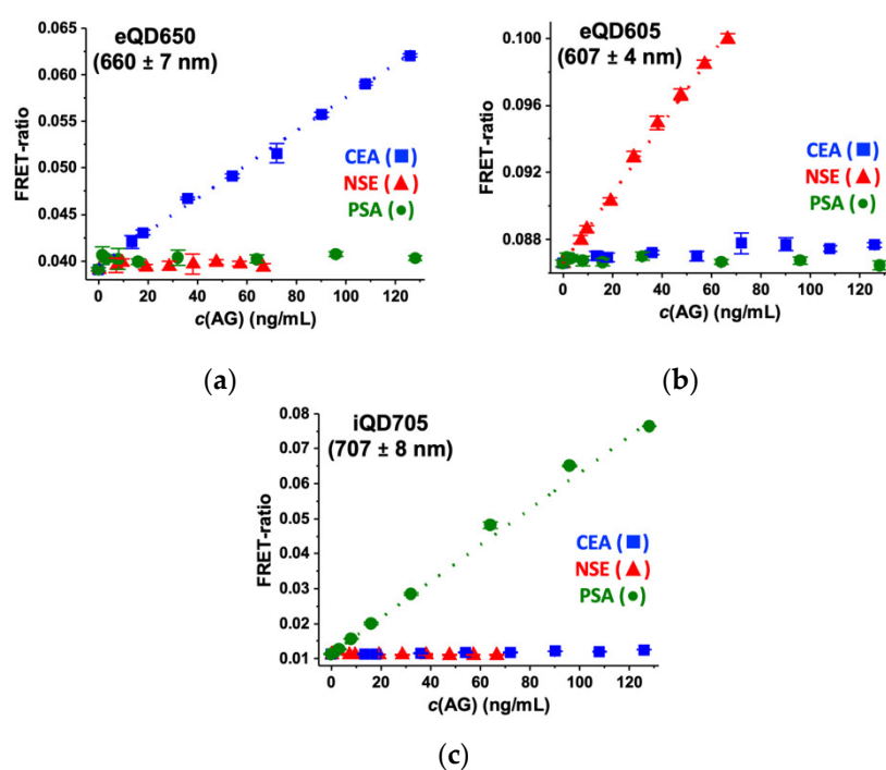
Figure 6. FRET immunoassay calibration curves of CEA, NSE, and PSA (all AB FRET pairs were present in all samples) to determine the optical crosstalk in: (a) the eQD650 detection channel for CEA; (b) the eQD605 detection channel for NSE; and (c) the iQD705 detection channel for PSA. Dotted lines show the linear fits of the AG-specific calibration curves that were used for the determination of LoDs.
