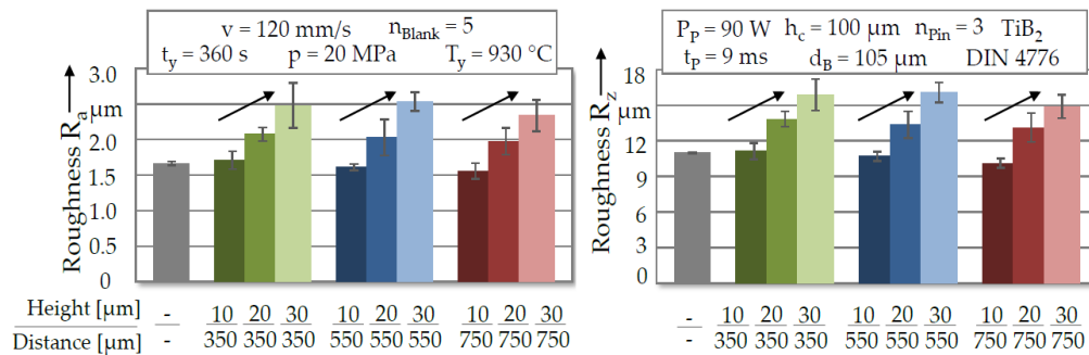
Figure 13. Tactile measurements of the worn blank topography according to the German Industrial Standard DIN 4476.
