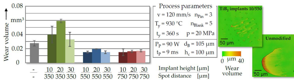
Figure 15. Quantified surface wear by using unmodified and laser-implanted tooling systems.
