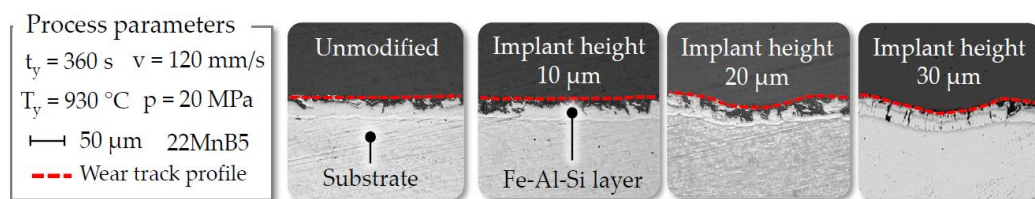
Figure 14. Cross-sectional preparations of the wear tracks.
