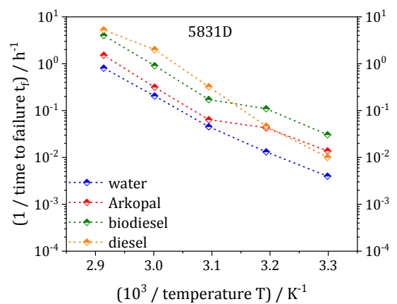
Figure 79: Arrhenius-like depiction of t_f (1 / t_f ) vs. temperature (1 / absolute temperature in K).
