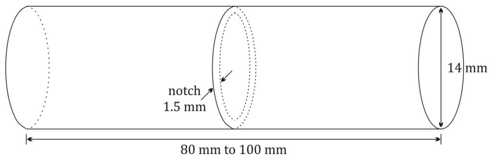
Figure 13: Configuration of CRB test specimen according to [115].
