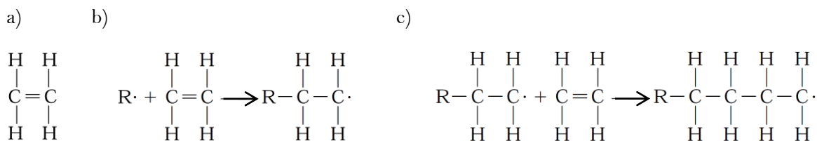
Figure 1: Formal polymerization process schematically depicted for initiator \text{R}\cdot and ethylene; a) ethylene monomer, b) reaction of initiator \text{R}\cdot to ethylene, c) transfer of active site to successive monomer end (after [18]).
