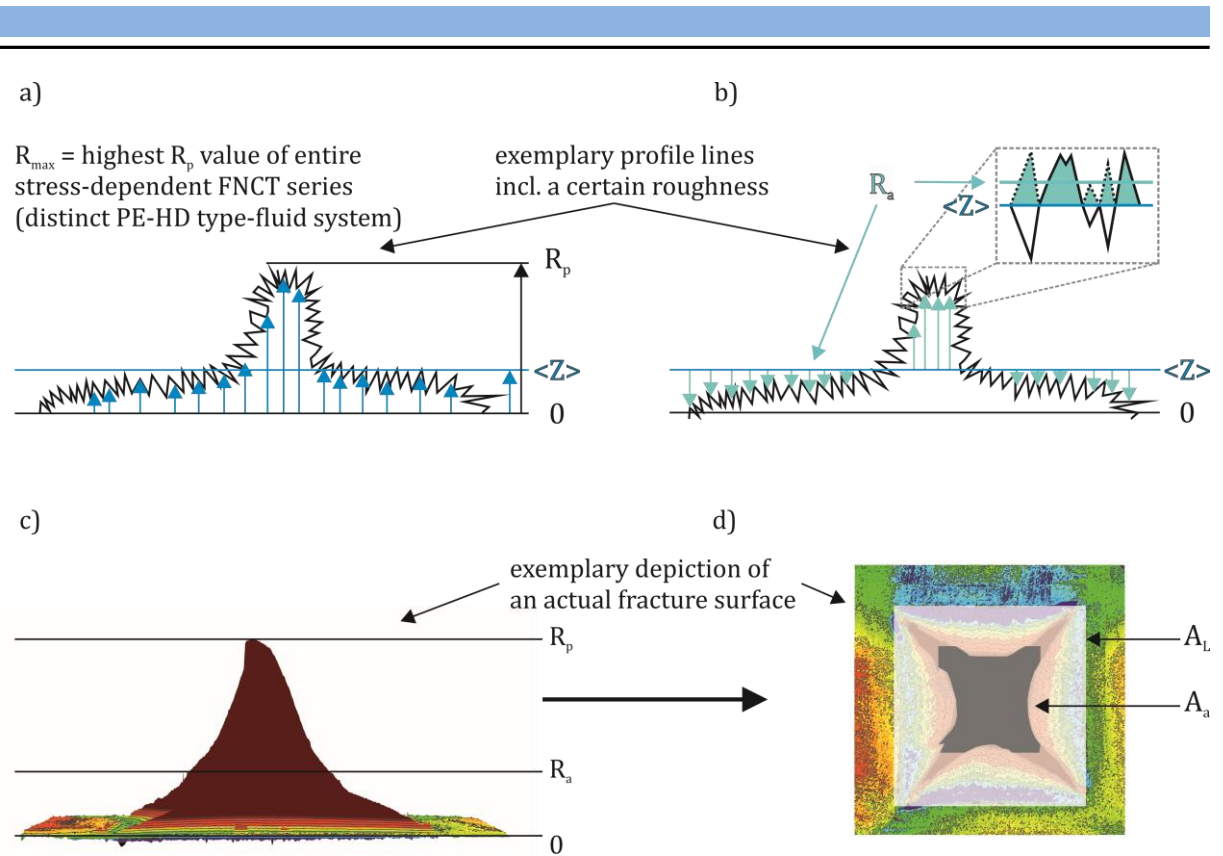
Figure 82: Schematic depiction of parameters used in the criterion of brittleness B, a) exemplary profile line describing R_p , R_{max} and \langle Z \rangle , b) exemplary profile line showing R_a , c), d) exemplary depiction of an actual fracture surface (ductile) with R_p , R_a , A_L and A_a .
