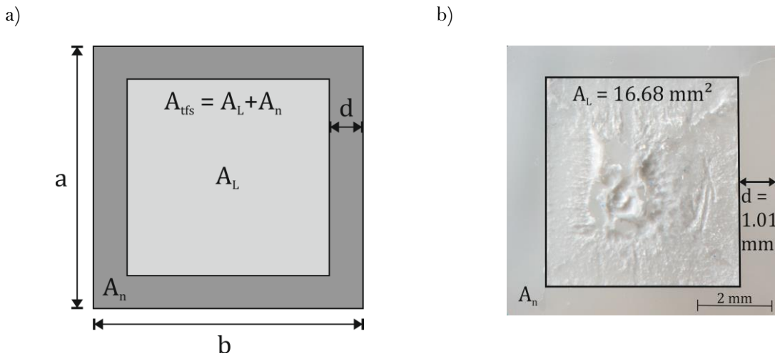
Figure 25: a) Schematic projection of the initial residual cross-section after notching, A_L : ligament area, d = d_{\text{notch}} : notch depth, A_n : notch area, A_{\text{tfs}} : area of total fracture surface, a , b : length and width (edge lengths) of FNCT specimen; b) example of exact determination of d and A_L employing light microscopy measurement tools.
