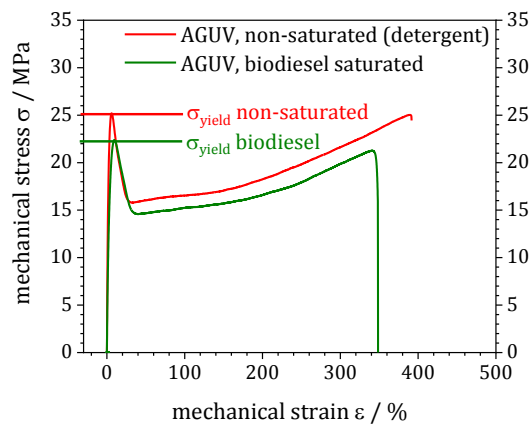
Figure A1.84: Tensile test results of non-saturated and biodiesel saturated AGUV specimens.
