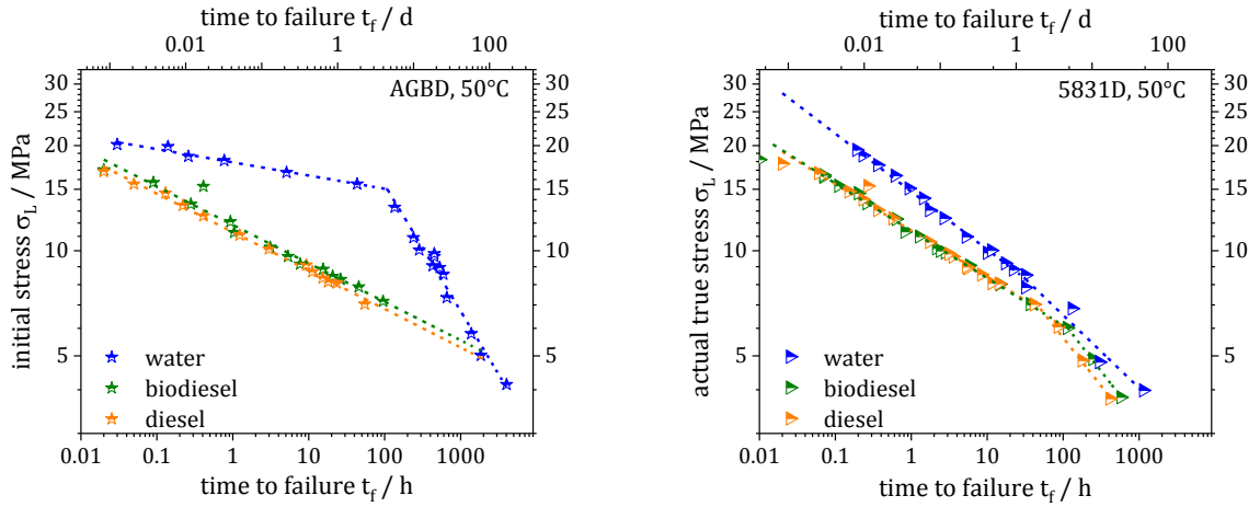
Figure B2.90: FNCT time to failure values t_f of AGBD (a) and 5831D (b) in water, biodiesel and diesel, each over a large range of actual applied stresses at 50°C (depiction in accordance with ISO 16770 [13]).
