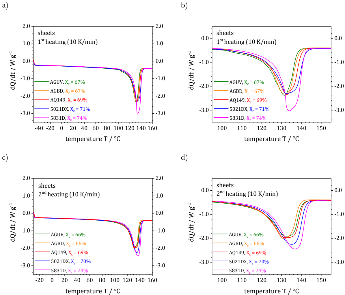
Figure 36: DSC data of the first and second heating in a temperature range of -50^{\circ}C to 160^{\circ}C (a) and -30^{\circ}C to 160^{\circ}C (c) with a heating rate of 10 K/min for 1 mm thick specimens, b), d) extracted data in the melting temperature range ( 95^{\circ}C to 155^{\circ}C ).
