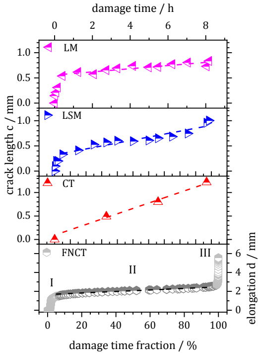
Figure 64: Average crack lengths and crack growth rates determined from the different imaging techniques compared to FNCT elongation data.
