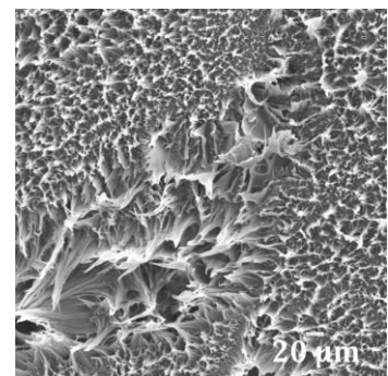
Figure B3.95: SEM fracture surfaces for fluid variation of AQ149 (air, Arkopal, diesel), FNCT specimens measured at 50°C, magnifications 30x, 200x and 500x (left to right), respectively.
