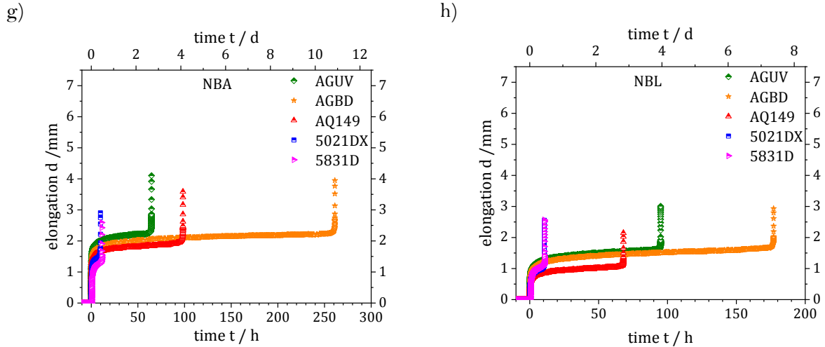
Figure 55: FNCT elongation data with \sigma_L \approx \sigma_n = 9 \text{ MPa} and 50^\circ\text{C} for each combination of PE-HD type and fluid.
