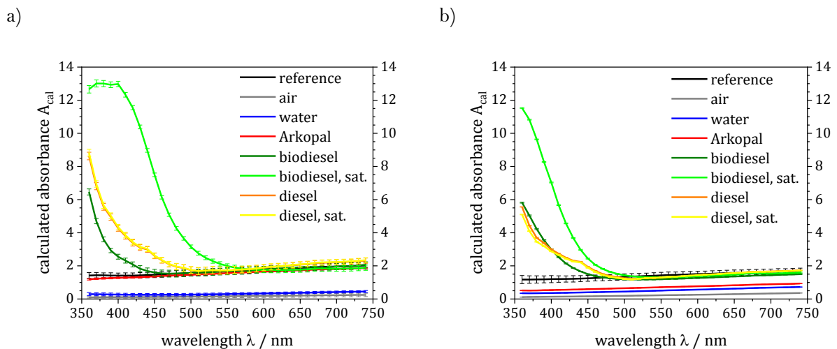
Figure 44: Calculated absorbance A_{cal} in dependence on wavelength \lambda (Kubelka-Munk function) for a) AGUV and b) 5021DX.
