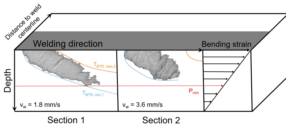
Figure 12. Schematic illustration of the limiting factors of hot crack formation in the two sections. Section 1: The crack length is limited by T_{BTR,min,1} and T_{BTR,max,2} . The crack depth is limited by P_{min} . Section 2: The crack length is limited by the weld centreline and the crack depth by T_{BTR,min,1} .
