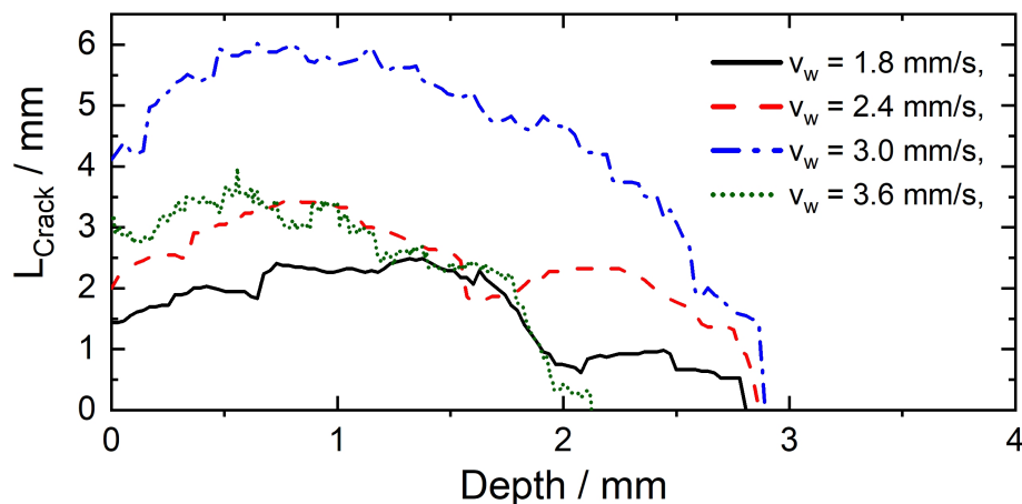
Figure 10. Distance L_{Crack} between the two fitted ellipses for MVT testing in Varestreint mode of Cr8Ni6 LTT weld filler material.
