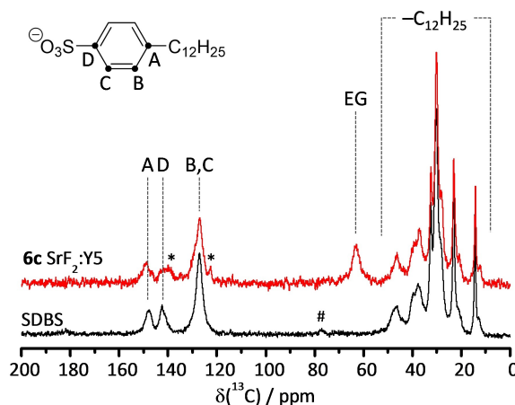
Figure 3. 1 H- 13 C CP MAS NMR spectra of neat SDBS and 6c SrF 2 :Y5 powder. EG: ethylene glycol, *: spinning side band, #: unknown impurity. The C 12 H 25 chain is a mixture of isomers.
