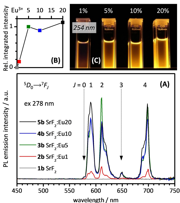
Figure 5. A: Photoluminescence spectra of 0.4 M SrF 2 :Eu 3+ in cyclohexane, excitation of aromatic system at 278 nm. B: Integrated emission intensity relative to SrF 2 :Eu5. C: Illumination of the sols at 254 nm.
