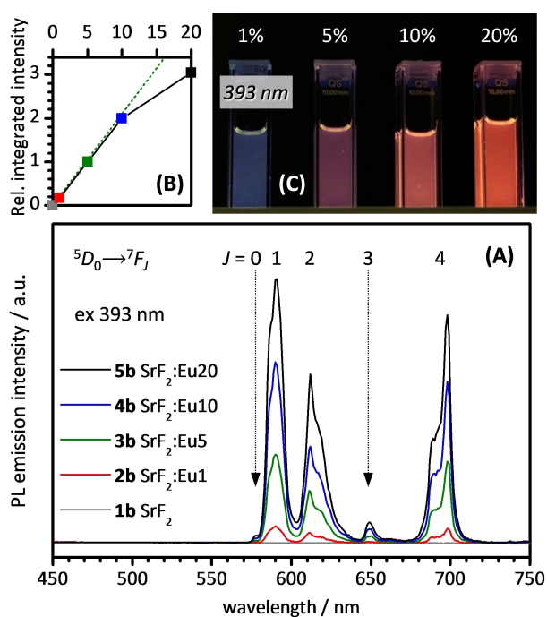
Figure 4. A: Photoluminescence emission spectra of 0.4 M SrF 2 :Eu 3+ in cyclohexane, direct excitation of Eu 3+ at 393 nm. B: Integrated emission intensity relative to SrF 2 :Eu5. C: Sols illuminated at 393 nm.
