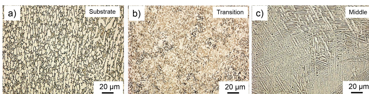
Figure 6. Typical micrographs obtained (a) in the substrate, (b) in the transition zone close to the substrate, (c) in the center of the WAAM part.
