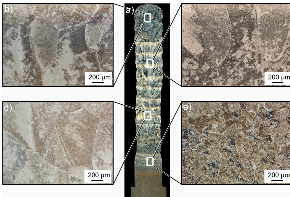
Figure 5. (a) Micrograph showing prior \beta -Ti grains in the middle section of the sample with enlarged view for (b) top of WAAM part, (c) and (d) middle height of WAAM part, (e) transition region between WAAM and forged parts.
