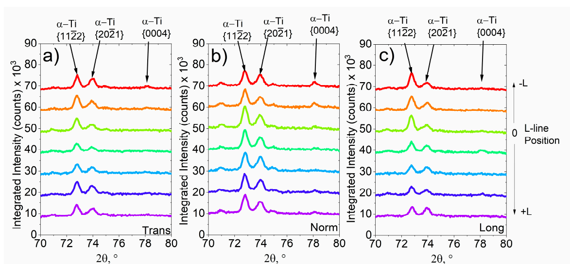
Figure 8. Diffraction patterns along the L-line for (a) transversal component, (b) normal component, (c) longitudinal component.
