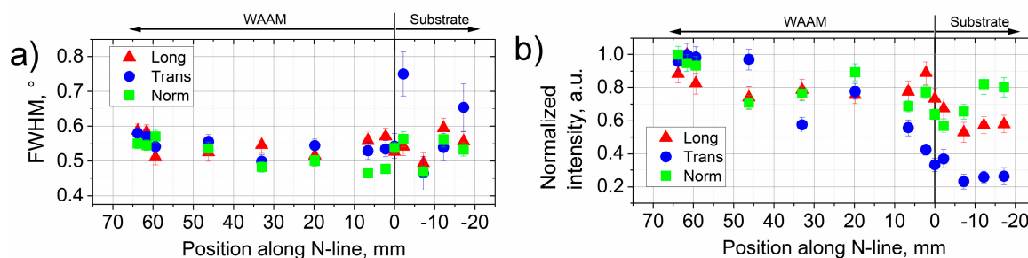
Figure 10. (a) FWHM and (b) normalized integrated intensity of the 11\bar{2}2 -Ti diffraction peak along the build direction.
