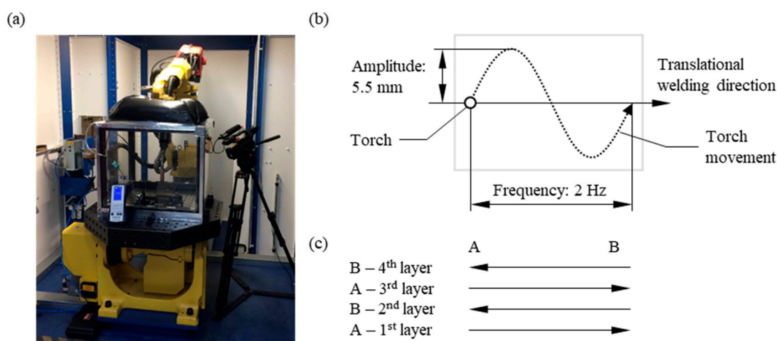
Figure 3. For the WAAM process (a) used WAAM machine, (b) applied sinus wave movement and (c) swapping of the starting point each layer.
