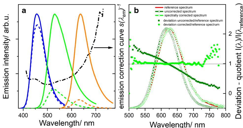
Fig. 1 Determination of the spectral characteristics of a fluorescence microscope and its validation. a Fluorescence emission spectra of solutions of the 3 spectral fluorescence standards dye C, dye D, and dye E (dashed lines: measured with the CLSM microscope FV1000; solid lines: normalized reference spectra), and the calculated emission correction curve s(\lambda_{em})^{-1} . b Comparison of the emission spectrum of a solution of the validation dye Y [12, 33] as measured with the CLSM
