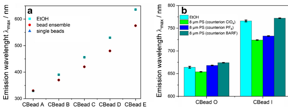
Fig. 3 a Encapsulation-induced hypsochromic shifts of the emission maxima of the Kit fluorophores in 8- \mu\text{m} PS beads as compared with solutions of the Kit dyes in ethanol underlining the effect of the surrounding matrix on the spectral features of the encapsulated fluorophores; standard deviations derived either from the wavelength accuracy of the respective fluorescence instrument used for the measurements or from the
