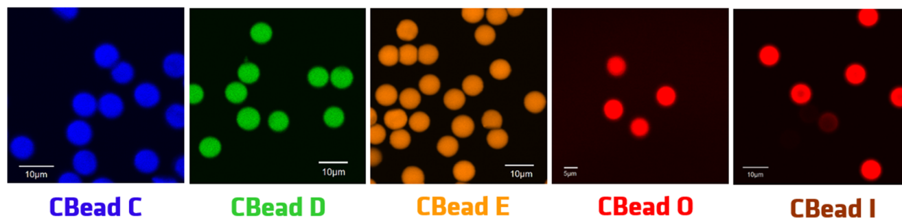
Fig. 4 Microscopy images of fluorophore-loaded 8 \mu\text{m} -sized PS beads (UPLSAPO 60x; excitation at 355 nm (CBead C), 488 nm (CBead D), 515 nm (CBead E), and 633 nm (CBead O and CBead I)
