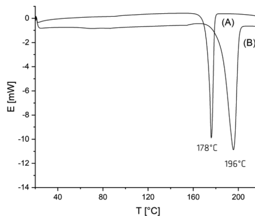
Fig. 2 DSC measurement of (A) no. 4A, Table 1 after precipitation into ligroin followed by annealing at 160 °C for 1 day, (B) no. 4B, Table 1.
