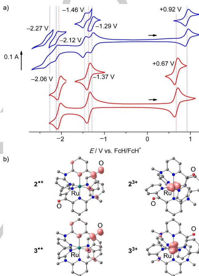
Figure 2. a) Cyclic voltammograms of 2 [PF 6 ] 2 (blue) and 3 [PF 6 ] 2 (red), 1 mM in acetonitrile, 0.1 M [tBu 4 N][PF 6 ] and b) DFT optimized geometries and spin densities (isosurface at 0.01 a. u.) of the radical cations 2 •+ and 3 •+ and the ruthenium(III) complexes 2 3+ and 3 3+ .
