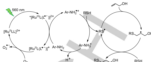
Scheme 3. Photocatalytic radical thiol-ene click reaction utilizing the (green) light-induced reductive quenching pathway of [\text{RuLL}]^{2+} = 2^{2+} , 3^{2+} and [\text{Ru}(\text{bpy})_3]^{2+} mediated by p -toluidine ( \text{Ar} = p\text{-C}_6\text{H}_4\text{-CH}_3 ) according to ref. [71] ( \text{R} = \text{CH}_2\text{-CHNH}_2\text{Boc-COOCH}_3 ).
