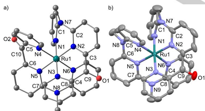
Figure 1. a) Molecular structure of \mathbf{2}^{2+} determined by DFT geometry optimization and b) \mathbf{3A}^{2+} determined by single crystal XRD, ellipsoids set at 50 % probability. Hydrogen atoms are omitted for clarity.
