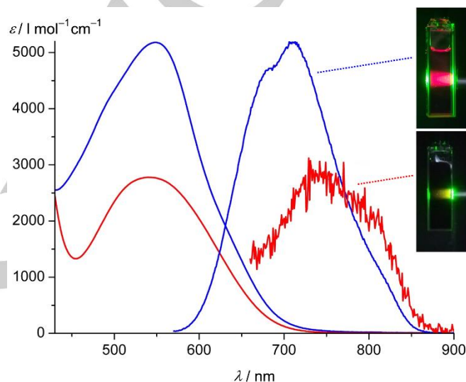
Figure 4. UV/Vis/NIR absorption and emission spectra (scaled to the respective MLCT absorption band) of 2[\text{PF}_6]_2 (blue) and 3[\text{PF}_6]_2 (red) in acetonitrile at 298 \text{ K} ( \lambda_{\text{exc}} = 544 \text{ nm} ). The photos display cuvettes of acetonitrile solutions of 2[\text{PF}_6]_2 and 3[\text{PF}_6]_2 under irradiation with green light ( 560 \text{ nm} ).
