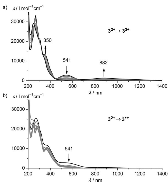
Figure 3. UV/Vis/NIR absorption spectra of 3[\text{PF}_6]_2 in acetonitrile with 0.1 \text{ M } [^t\text{Bu}_4\text{N}][\text{PF}_6] at 298 \text{ K} collected during a) electrochemical oxidation and b) electrochemical reduction.
