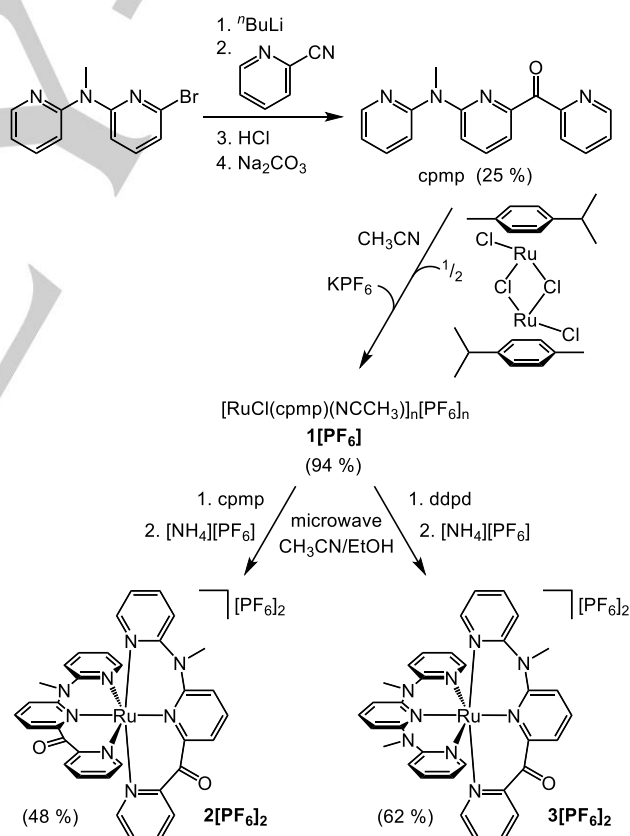
Scheme 2. Synthesis of the ligand cpmp and its ruthenium(II) complexes 1 [PF 6 ] n , 2 [PF 6 ] 2 and 3 [PF 6 ] 2 .
