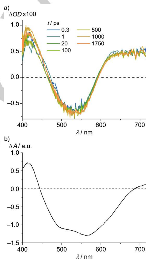
Figure 5. a) fs-Transient absorption spectra of 2 [PF 6 ] 2 in acetonitrile at different delay times after excitation at 540 nm at 293 K and b) estimated difference spectrum [67] derived from absorption spectra of 2 2+ , 2 3+ and 2 2+ , prepared electrochemically in acetonitrile with 0.1 M [ 18 Bu 4 N][PF 6 ] at 298 K by “scaled [ \frac{1}{2}(\mathbf{2}^{\mathbf{3}+} + \mathbf{2}^{\mathbf{2}+}) - \mathbf{2}^{\mathbf{2}+} ]”.
