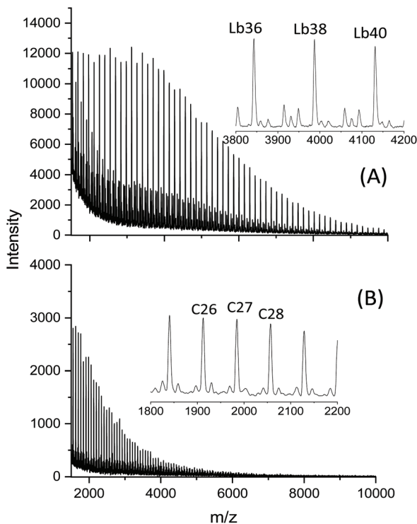
Fig. 3 MALDI-TOF mass spectra of poly(L-lactide)s polymerized with pentafluorophenol+SnOct 2 in bulk: (A) 160 °C/1 h with In/Cat = 2000/1, (B) 160 °C/4 h with In/Cat = 1000/1 (reprinted from ref. 27 with permission of Wiley).
