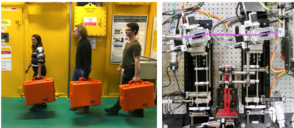
Fig. 1. The two crystal stages and the central sample stage can be transported together with a range of accessories in the three flight cases shown on the left-hand side. A top-down view of the USAXS module as installed at the beamline, with the X-ray beam drawn in purple, travelling from left to right through the two channel-cut Si(220) crystals.
