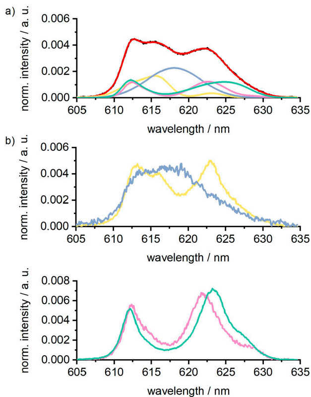
Figure 5. a) Gaussian fitting (red) of the measured {}^5D_0-{}^7F_2 emission band of Eu(III) (—) in CSI with HCA after 28 d hydration time (delay time t_d = 1000 \mu\text{s} , \lambda_{\text{ex}} = 394 \text{ nm} ) and b) {}^5D_0-{}^7F_2 emission band of the references (yellow: Eu(III) in portlandite ( t_d = 200 \mu\text{s} ), blue: Eu(III)-carbonate ( \text{pH} = 12.0 , t_d = 1013 \mu\text{s} ), magenta: Eu(III) in C–S–H ( C/S = 1.4 , \text{pH} = 12.6 , t_d = 1730 \mu\text{s} ), and green: Eu(III) in ettringite ( \text{pH} = 12.6 , t_d = 1730 \mu\text{s} )).
