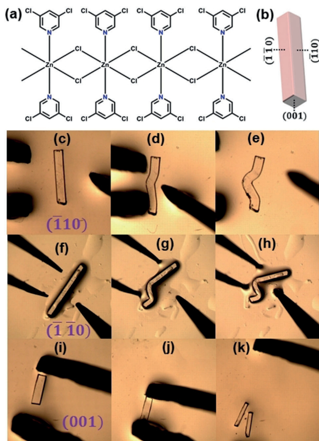
Figure 1. a) Chemical structure of [\text{Zn}(\mu\text{-Cl})_2(3,5\text{-dichloropyridine})_2]_n ( 1 ). b) Crystal face indices of a crystal of 1 determined by single-crystal X-ray diffraction. c–k) Optical microscopic photographs of single crystals of 1 undergoing three-point bending. Tweezers were used to restrain the crystal ends and a needle exerted a force between the restrained ends. Plastic bending along the major crystallographic faces (c–e) for (\bar{1}10) and (f–h) for (\bar{1}\bar{1}0) . i–k) Brittle fracture when stressed along the (001) crystallographic face.
