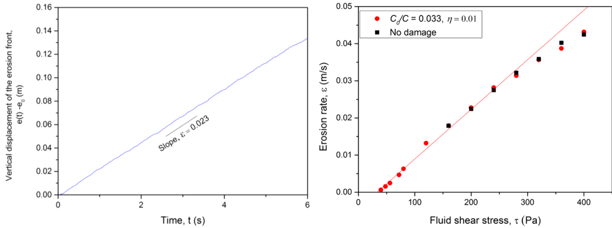
Fig. 18. Soil erosion under homogeneous shear flow conditions. Left: Evolution of the erosion front with time for a cohesive bond strength of C = 3\text{ N} (basic cohesion scheme without damage model) and a fluid flow involving \nu = 2 \cdot 10^{-4} \text{ m}^2/\text{s} , U_0 = 5 \text{ m/s} and e_0 = 5 \text{ mm} . Right: Variation of erosion rate \varepsilon with the prescribed fluid shear stress \tau upon consideration of transient damage (damage threshold C_0 = 0.033 \cdot C and characteristic time \eta = 0.01 ). The solid line represents a linear fit of the damage data (red points) in the stress range up to 300 Pa. (For interpretation of the references to colour in this figure legend, the reader is referred to the web version of this article.)
