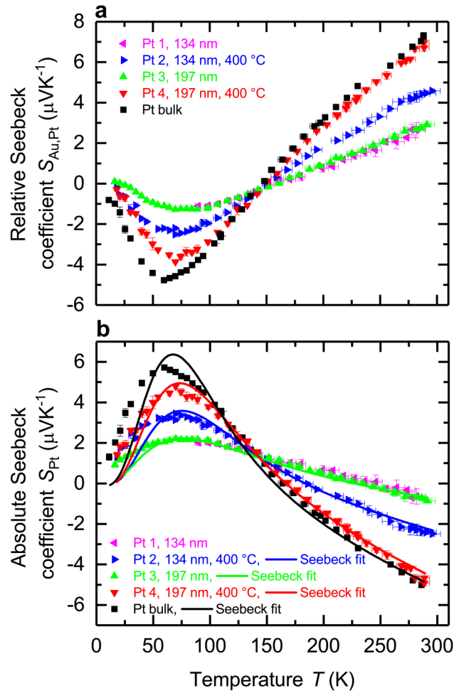
FIG. 5. Relative and absolute Seebeck coefficient of thin platinum films as sputtered and with heat treatment and bulk material. (a) Relative Seebeck coefficient S_{Au,Pt} of platinum relative to a bulk gold wire with a diameter of 25 \mu\text{m} as a function of the bath temperature T . (b) Absolute Seebeck coefficient S_{Pt} of platinum as a function of the bath temperature T . The corresponding solid lines represent the Seebeck fit of the data. Absolute Seebeck coefficient of bulk gold S_{Au} was taken from Ref. 28.
