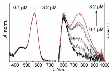
Figure 10. Normalized absorption and fluorescence spectra ( \lambda_{\text{ex}} = 520 \text{ nm} ) of aqueous solutions of DHNBDP-Me at different concentrations from 0.1 \mu\text{M} (solid black) to 3.2 \mu\text{M} (red) with steps of 0.2, 0.4, 0.8 and 1.6 \mu\text{M} .
