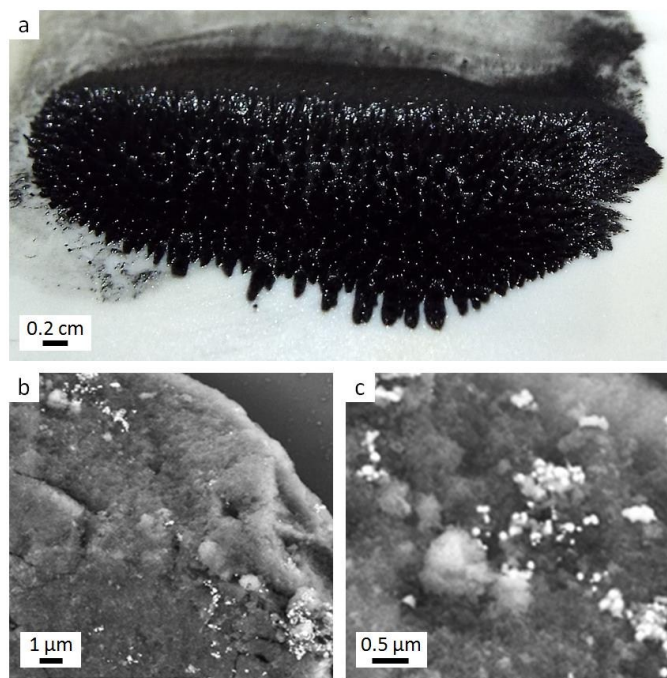
Fig. 7 a) Image of \text{Fe}_3\text{C} ferrofluid, showing characteristic 'spikes' of the fluid following magnetic field lines. b/c) SEM images taken with a backscattered electron detector showing bright \text{Fe}_3\text{C} nanoparticles on \text{SiO}_2 .
