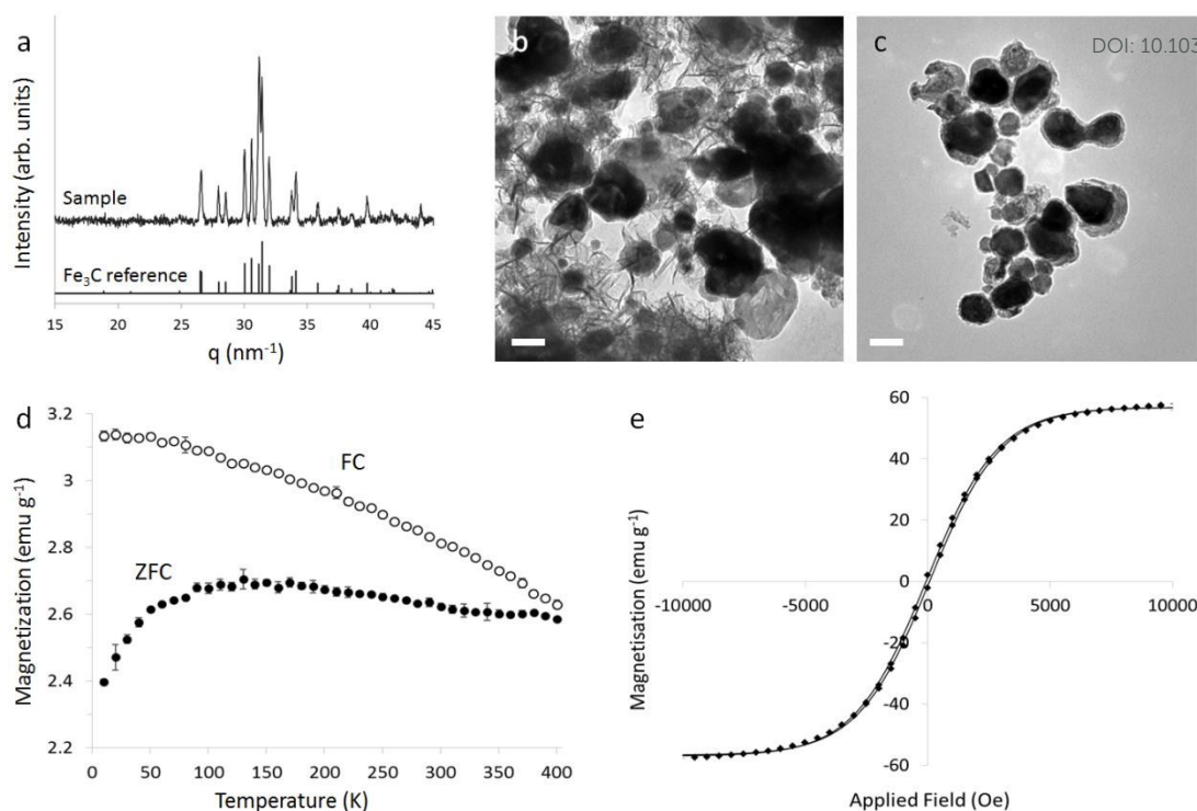
Fig 5 a) XRD pattern of \text{Fe}_3\text{C} sample after EDTA treatment, with a reference pattern for \text{Fe}_3\text{C} . TEM images of \text{Fe}_3\text{C} sample b) before and c) after \text{H}_2\text{O}_2 treatment to remove excess amorphous carbon (scale bar = 100 nm). d) Temperature dependence of the zero-field-cooled (ZFC) and field-cooled (FC) magnetization of a packed powder of \text{Fe}_3\text{C} from 10–400 K under an applied field of 100 Oe. NB: measurements could not be made above 400 K in the given apparatus. e) Plot of the field dependence of isothermal magnetization at 400 K with data fit to a Boltzmann distribution.
