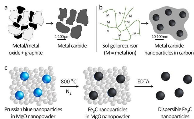
Fig. 1 Schematics of a) conventional solid-state synthesis of metal carbide powders, b) sol-gel synthesis of metal carbide nanoparticles from mixtures of metal salts with organic precursors such as polymers. c) Schematic of new method of 'nanocasting' dispersible Fe 3 C nanoparticles in MgO nanopowder.
