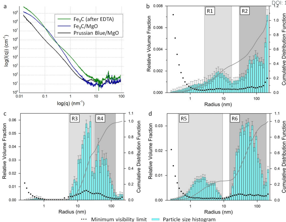
Fig 6 a) Small- and wide-angle X-ray scattering data fits for samples of Prussian blue/MgO, Fe 3 C/MgO and Fe 3 C. Particle size histograms coupled with visibility limits (black dots, left y-axis) and cumulative distribution functions (right y-axis) for b) Prussian blue/MgO, c) Fe 3 C/MgO and d) Fe 3 C.
