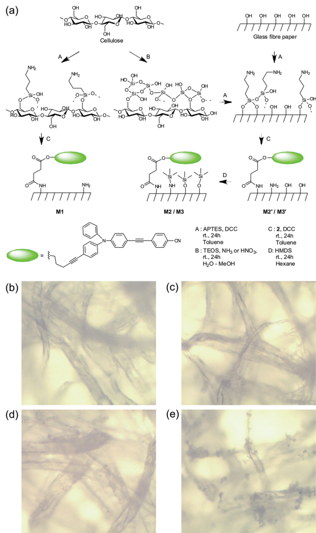
Fig. 3 (a) Scheme representing the preparations of the different test strips M1 , M2' , M2 , M3' , and M3 . Microscopy photographs of cellulose without coating ( b ) and silica-coated cellulose strip obtained ( c ) under acidic conditions ( \text{HNO}_3 , #4), ( d ) with 0.7 equivalents of ammonia vs. TEOS (#6) and ( e ) 0.2 equivalents of ammonia vs. TEOS (#10).
