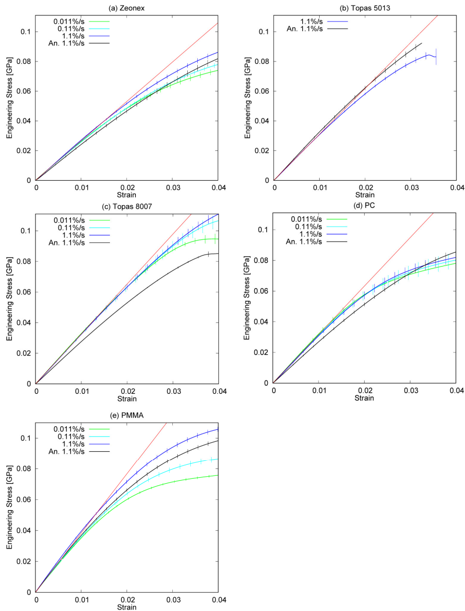
Fig. 3. Engineering stress, \sigma = F / A ( F is the drawing force and A = N / \sum_1^N 1 / A_i is the average cross sectional area of the fiber), as a function of engineering strain, \epsilon = (L - L_0) / L_0 ( L is the current length of the fibre and L_0 the initial length) in the elastic region for the un-annealed and annealed POFs strained at different straining rates ( \dot{\epsilon} = d\epsilon / dt = (1 / L_0) \cdot dL / dt ). The un-annealed POFs were strained at rates, \dot{\epsilon} , of 0.011%/s. (green line), 0.11%/s (light blue line) and 1.1%/s (dark blue line). The annealed POFs were strained at a rate, \dot{\epsilon} , of 1.1%/s (black line). The error bars represent \pm one standard deviation. The red line is the linear elasticity, based on an overall average for the un-annealed fibres. Figure 3(a): Zeonex 480R POFs. Figure 3(b): Topas 5013S-04 POFs. Figure 3(c): Topas 8007S-04 POFs. Figure 3(d): PC Makrolon LED2245 POFs. Figure 3(e): PMMA (GEHR) POFs.
