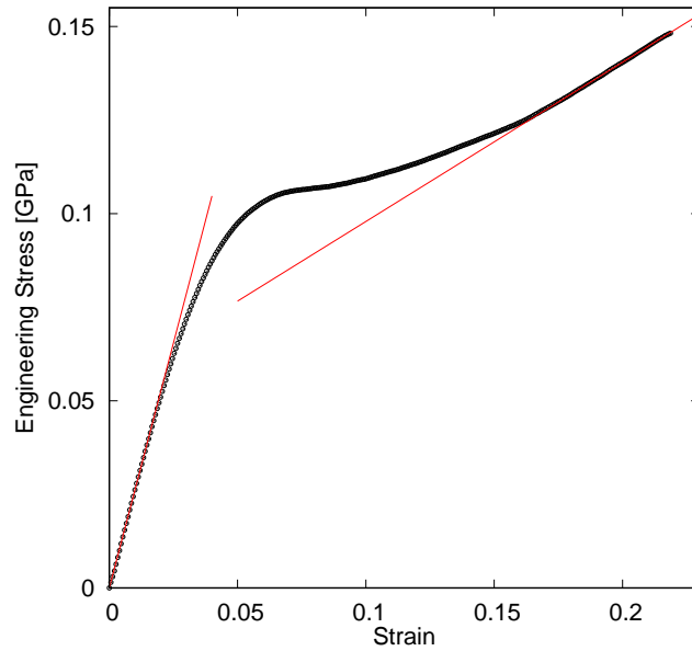
Fig. 1. Engineering stress, \sigma = F / A ( F is the drawing force and A = N / \sum_1^N 1 / A_i is the average cross sectional area of the fiber), as a function of engineering strain, \epsilon = (L - L_0) / L_0 ( L is the current length of the fibre and L_0 the initial length), for an un-annealed Zeonex fibre. The straining rate ( \dot{\epsilon} = d\epsilon / dt = (1 / L_0) \cdot dL / dt ) is 1.1%/s.
