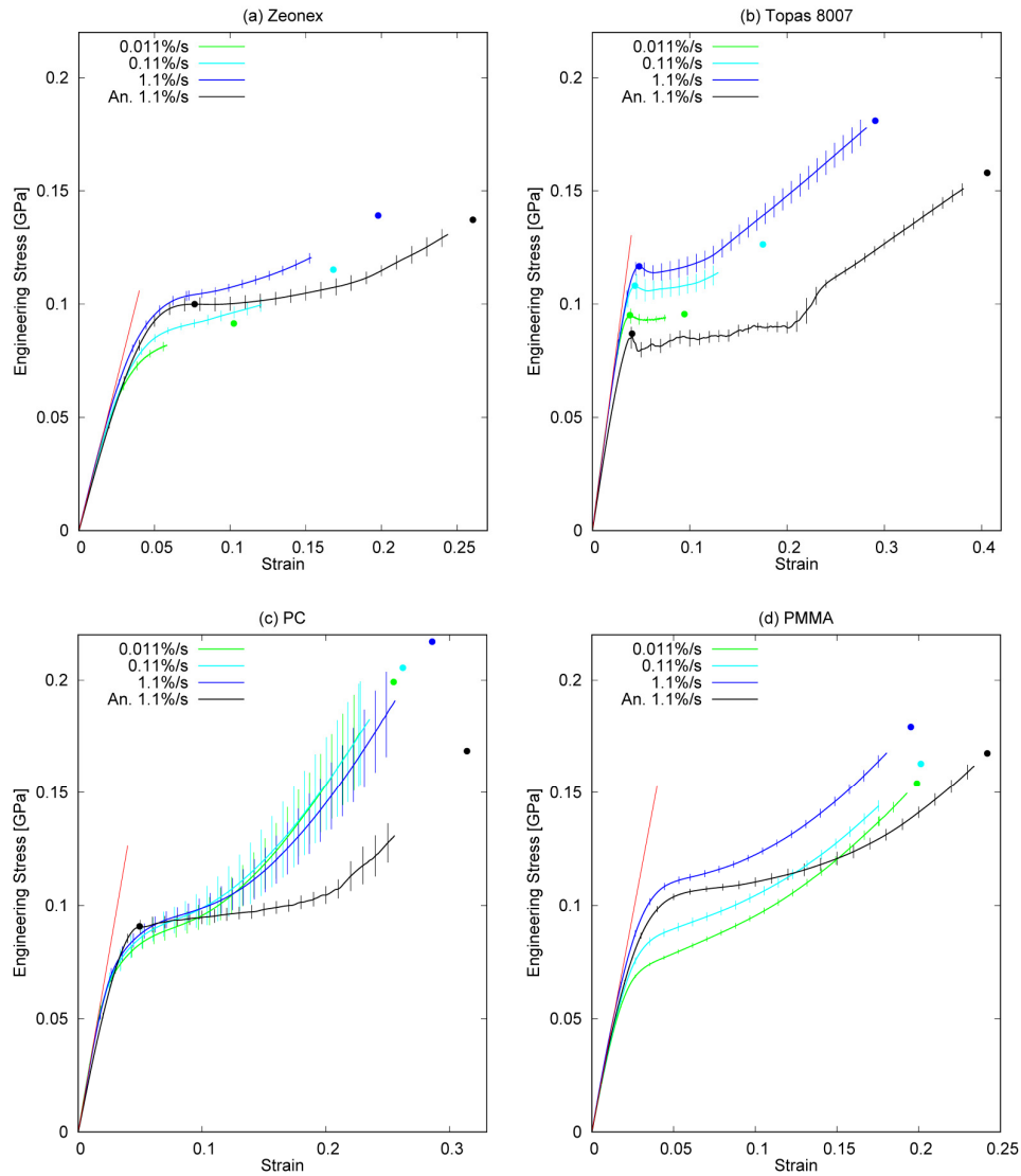
Fig. 4. Engineering stress, \sigma = F / A ( F is the drawing force and A = N / \sum_1^N 1 / A_i is the average cross sectional area of the fiber), as a function of engineering strain, \epsilon = (L - L_0) / L_0 ( L is the current length of the fibre and L_0 the initial length). These are the full stress-strain curves of the un-annealed and annealed POFs strained at different straining rates. The un-annealed POFs were strained at strained at rates, \dot{\mathcal{E}} ( \dot{\mathcal{E}} = d\epsilon / dt = (1 / L_0) \cdot dL / dt ) of 0.011%/s. (green line), 0.11%/s (light blue line) and 1.1%/s (dark blue line). The annealed POFs were strained at a rate of, \dot{\mathcal{E}} , of 1.1%/s (black line). The error bars represent \pm one standard deviation. The red line is the linear elasticity, E (defined in Fig. 2), based on an overall average for the un-annealed fibres. The curves are all terminated at the lowest (engineering) strain at break values observed in the experiments. The bullets represent the average yield (the first maximum on the stress-strain curve) and break points (final point on the stress-strain curve), based on the average data for the corresponding fibre type. The bullets have the same colour as the corresponding lines. The average yield points have been shown on the as the bullets on the stress strain lines. The average break of the POFs has been shown as the bullets after the stress strain lines. Figure 4(a): Zeonex 480R POFs. Figure 4(b): Topas 8007S-04. Figure 4(c): PC Makrolon LED2245 POFs. Figure 4(d): PMMA (GEHR) POFs.
