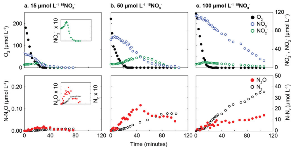
Fig. 1. The production and consumption of denitrification intermediates during dynamic incubations. Sediment columns were percolated with aerated seawater spiked with different starting concentrations of ^{15}\text{NO}_3^- and the production and consumption of denitrification intermediates was determined over time both while \text{O}_2 was still present and after the columns became anoxic. \text{N-N}_2 and \text{N-N}_2\text{O} concentrations are the total production of \text{N} as either \text{N}_2 or \text{N}_2\text{O} determined from the measured ^{29}\text{N}_2 and ^{30}\text{N}_2 or ^{45}\text{N}_2\text{O} and ^{46}\text{N}_2\text{O} concentrations. The inlays show the \text{NO}_2^- , \text{N-N}_2\text{O} and \text{N-N}_2 concentrations magnified 10 \times in comparison to the y-axis on the main plots (the x-axis remains 0–120 min).
