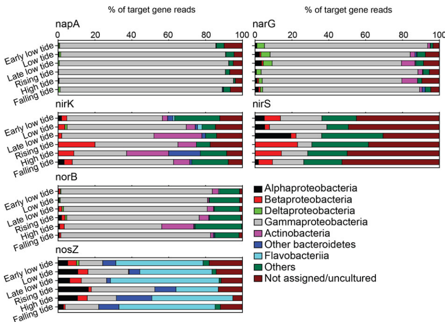
Fig. 4. Uneven taxonomic distribution of denitrification functional gene transcripts across a tidal cycle.
