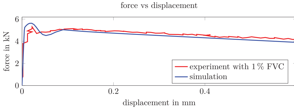
Figure 1. Experimental and numerical results of a uniaxial tension test on a dogbone specimen.
