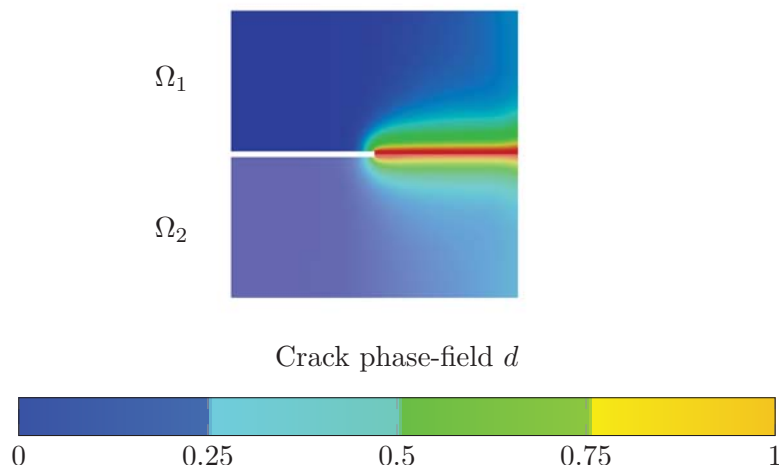
Figure 4. Crack phase-field at and u_y = 7.5 \mu\text{m} . Subdomain \Omega_1 opacity = 1.0. Subdomain \Omega_2 opacity = 0.5.
