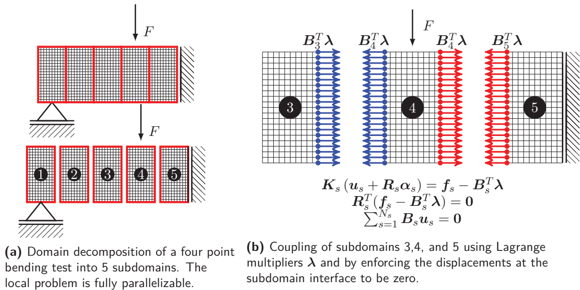
Figure 3. Finite element tearing and interconnecting method for a four point bending test.
