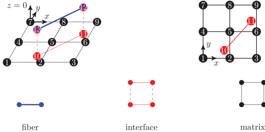
Figure 2. Bond between steel fibers and concrete matrix via an interface. The discretization of the concrete matrix is independent of the position and orientation of the fibers.
