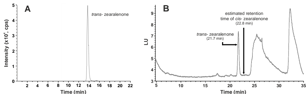
Figure 15. Chromatograms of corn oil no. 3 analyzed by (A) HPLC-MS/MS (Method A) and (B) DCHC-HPLC-FLD (Method B). The broad signals beginning at 24 min (Method B) are not caused by oil matrix but related to HPLC gradient (fast increase of solvent B (ACN) and reconditioning, respectively).
