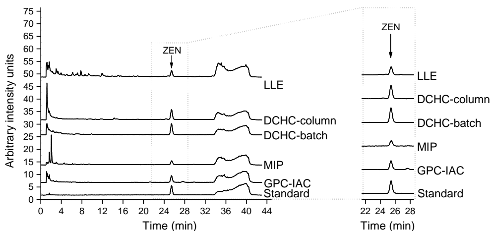
Figure 5. HPLC-FLD chromatograms of oil sample S2, a refined maize germ oil spiked with ZEN to a final content of 275 \mu\text{g}/\text{kg} , as analyzed by GPC-IAC, MIP, DCHC-batch, DCHC-column and LLE. The lowest trace corresponds to a ZEN standard in elution solvent.
