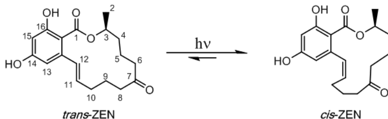
Figure 26. Photoisomerization of trans -ZEN to cis -ZEN at the double bond C11-C12.
