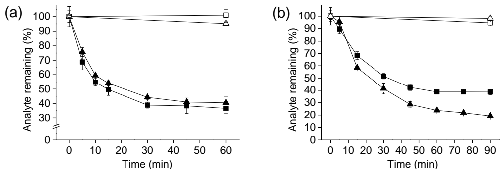
Figure 28. Depletion profile of 1 \mu M cis -ZEN (triangle) and trans -ZEN (square) in RLM (a) and HLM (b). The corresponding NADPH depleted controls clearly show the dependence of phase I metabolism of cis -ZEN (blank triangle) and trans -ZEN (blank square) on NADPH as cofactor. Error bars represent the standard deviation ( n = 3 for samples containing NADPH; n = 2 for controls).
