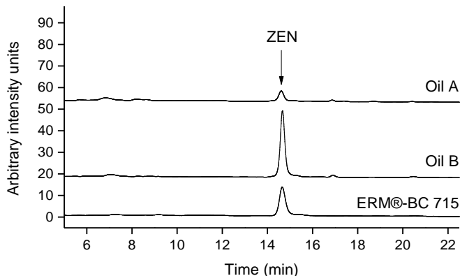
Figure 12. HPLC-FLD chromatograms of spiked maize germ oil A (100 \mu\text{g}/\text{kg} ; upper trace), maize germ oil B (602 \mu\text{g}/\text{kg} ; mid trace) and the provisionally certified reference material ERM ® -BC715 (362 \mu\text{g}/\text{kg} ; lower trace).
