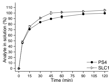
Figure 9. Time course of ZEN in the solvent supernatant upon decoupling from the hydrazine functionalized materials (n=3).
