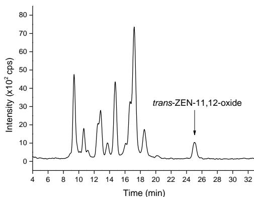
Figure 35. Extracted ion chromatogram ( m/z 333) obtained by incubation of 10 \mu\text{M} trans -ZEN with HLM and successive HPLC-ESI-MS analysis.
