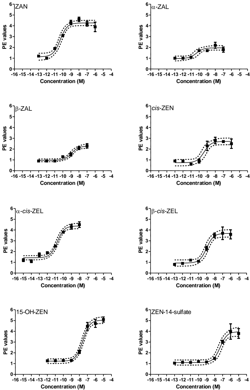
Figure 38. Concentration-response relationships for MCF-7 cells treated with ZEN congeners or 17 \beta -estradiol. Data points are expressed as means with error bars representing the standard deviation (n = 4). Dashed lines depict the 95 % confidence intervals.
