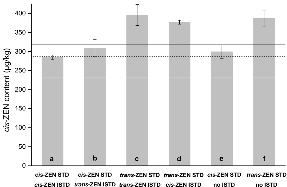
Figure 25. Determination of cis -ZEN in a spiked maize germ oil ( n = 4 ) by various quantification approaches (a - f). Error bars represent the standard deviation.
