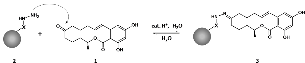
Figure 7. ZEN (1) and a hydrazine moiety (2) bound to a solid phase reversibly form a ZEN hydrazone (3).
