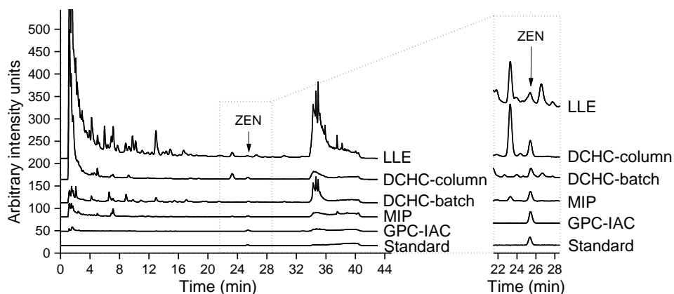
Figure 6. HPLC-FLD chromatograms of oil sample N1, a naturally ZEN contaminated virgin maize germ oil ( \omega_{ZEN} = 124 \pm 8 determined by LC-MS/MS), as analyzed by GPC-IAC, MIP, DCHC-batch, DCHC-column and LLE. The lowest trace corresponds to a ZEN standard in elution solvent.
