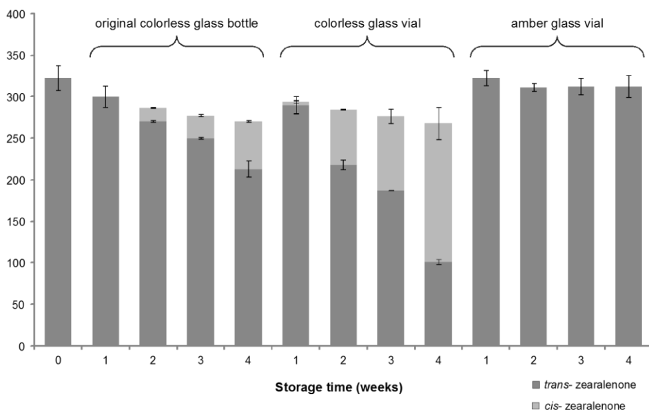
Figure 16. Isomerization of a naturally trans -zearalenone contaminated corn oil (no. 3) over 4 weeks of sunlight exposure (day-night-rhythm), analyzed by SIDA-HPLC-MS/MS (Method A). The mean values and their corresponding standard deviations are given based on three independent replicates ( n = 3 ).
