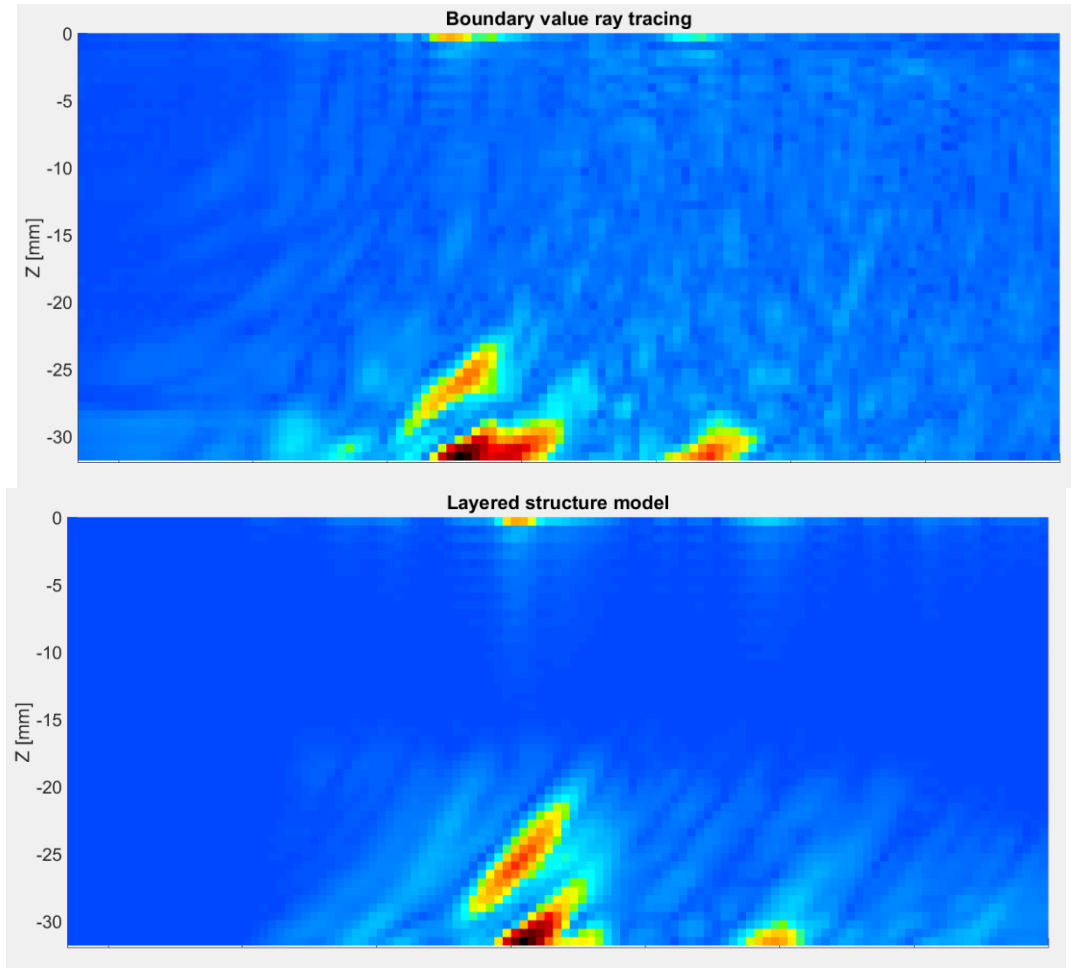
Fig. 3. Comparison of SAFT results using and the boundary value problem formulation (top) and a layer model with initial value ray tracing (bottom) for ray tracing.
