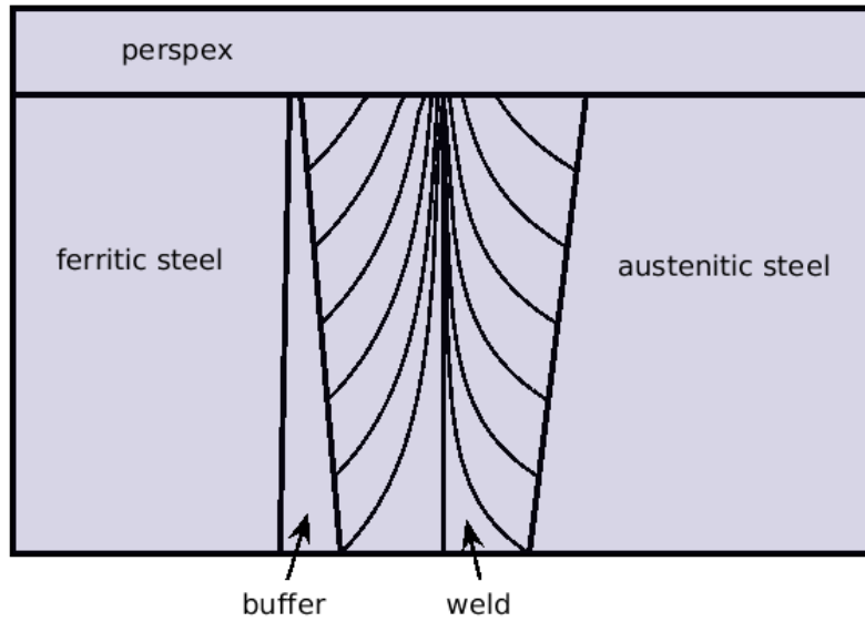
Fig. 1. Sketch of the considered geometry. The height of the weld is 32mm with an additional 6mm perspex layer. The buffer has a layback angle of 11^\circ and a constant crystal orientation of 82^\circ , the weld has a layback angle of 8^\circ and the crystal orientation given by the Ogilvy model with parameters T = (-0.5614, 0.9266) , a = (5.6574, 3.9685) , \eta = 1 . The extension of the weld is 9.945 mm at the top and (5.9825 mm, 7.17 mm) at the bottom, right and left of the weld center. The x-coordinates of the buffer are 10.7 mm left of the weld center at the top, and 11.39 mm at the bottom.
