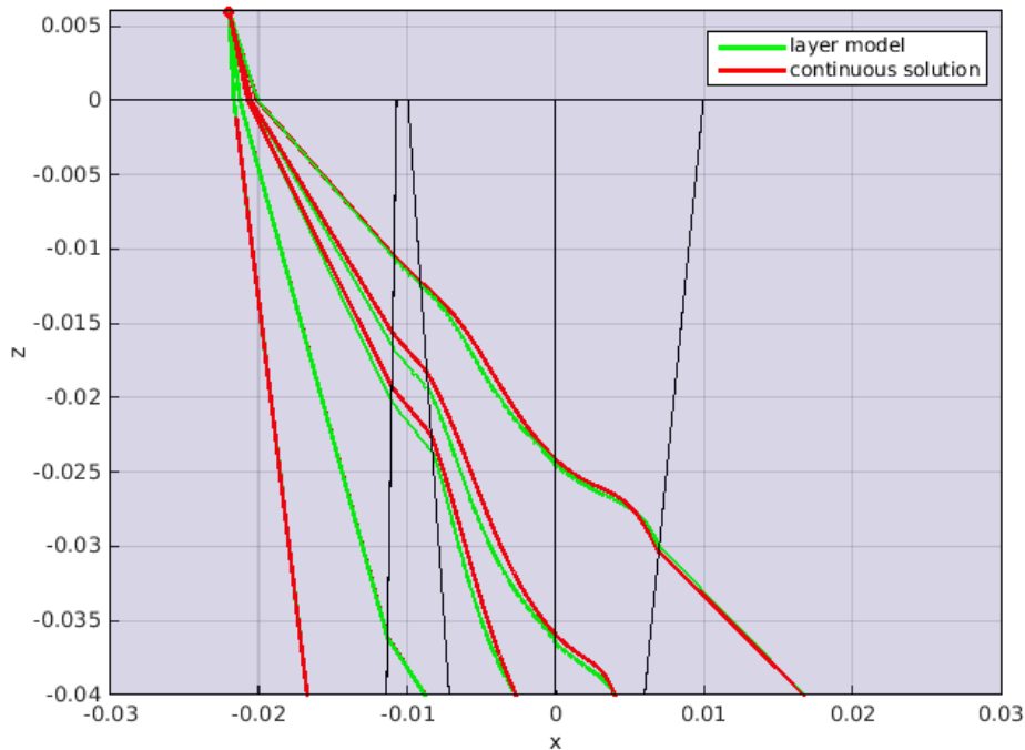
Fig. 2. Comparison of boundary value ray tracing using a layer model (green) and a continuous model for the for the grain orientation (red) along a cross section of the specimen. As expected, small differences between the layer model and the ODE solution are visible inside the weld.
