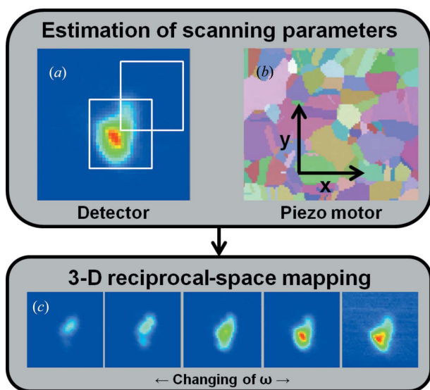
Figure 2 Schematic drawing of the experimental approach. After the estimation of the scanning parameters concerning the real-space ( b ) and the detector regions ( a ), maps ( x , y ) for each chosen incidence angle \omega in the vicinity of the hkl reflection were recorded ( c ).
