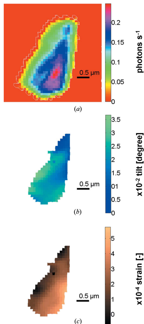
Figure 3 (a) Measured integral intensity of the 155 cubic reflection, showing the shape of a CuInSe 2 grain. (b) Calculated tilt-distribution map (orientational variance) of the measured grain. (c) Strain distribution map based on evaluated d_0 location. The data were acquired at an X-ray energy of 8.9 keV, a beam size of 100 \times 100 nm and a step size in the scan of 100 nm.
