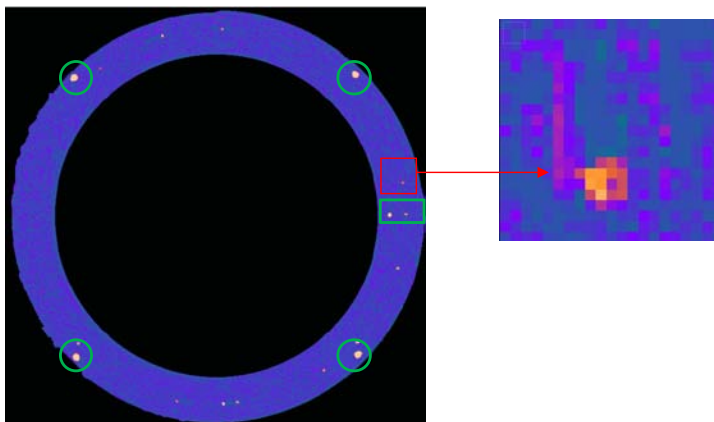
Figure 15: An example of an image of the canister lid (left) with an enlarged indication (right). Note : Marked in green are the indications resulting from screws used to lift and carry the lid (circles) and from the starting point of the measurement (rectangle), which the participants are taught to exclude from the evaluation.
