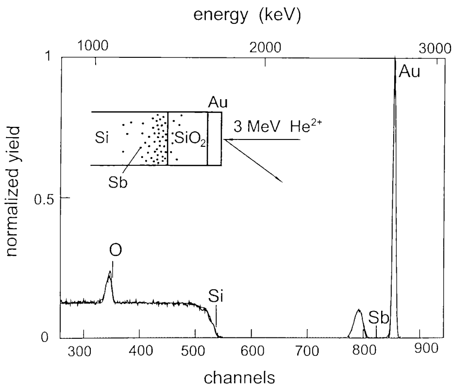
Figure 4: RBS spectrum of implanted Sb in Si with evaporated Au layer.
