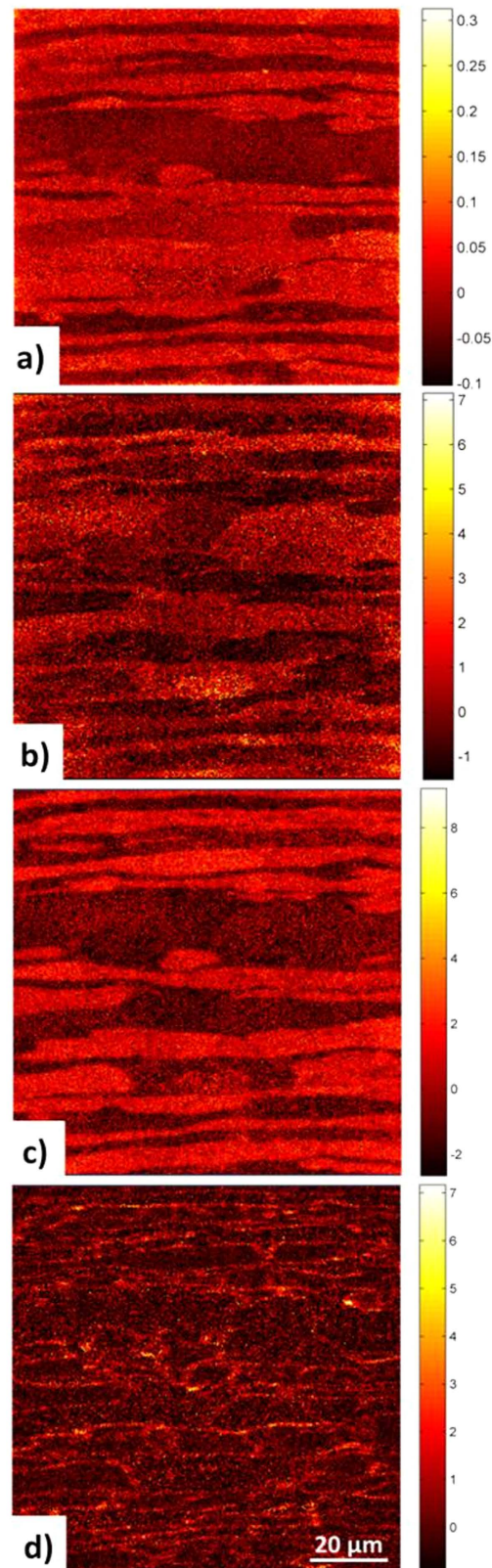
Figure 2. Principle component score images of the ToF-SIMS data sets acquired after 34 days of charging. (a) PC1 scores image for identifying phases using the positive ToF-SIMS data set acquired after 34 days of charging DSS with deuterium by using a peak list with secondary ions covering the main alloying elements. The bright regions represent the austenite phase (as proved by the loadings plot in shown Figure S2a). (b) PC1 scores image identifying locations rich in deuterium obtained from the negative SIMS data set acquired after 34 days and using the full peak list. Bright pixel indicate positive scores and correlate with the ferrite phase. (c) PC1 scores image obtained from the same data set but using a different peak list prepared to focus on carbides and
