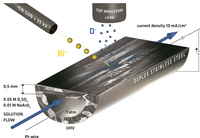
Figure 1. Schematic view of the unique design of the real time and in-situ deuterium permeation experiment within ultra-high vacuum chamber of the ToF-SIMS instrument. This set-up enables to monitor the deuterium distribution in the DSS microstructure at the polished vacuum exposed surface of the charging cell made from 2205 DSS. Deuterium becomes visible after permeation through a 0.5 mm thick DSS sheet.
