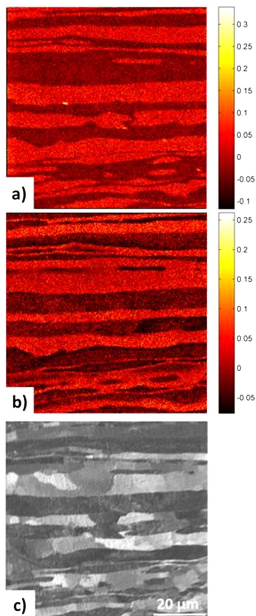
Figure 3. Principle component score and secondary electron images of the ToF-SIMS data sets acquired after 37 days of charging. (a) PC1 scores image obtained from the positive SIMS data set acquired after 37 days of charging DSS and used to identify phases in the DSS microstructure. A fresh region of interest (ROI) has been selected. The bright regions represent the austenite phase (as shown in the loading plot in Figure S2a). (b) PC1 scores image related to locations rich in deuterium. The image was generated by PCA of a negative ToF-SIMS image data set obtained after loading with deuterium for 37 days. The bright deuterium-rich areas have positive scores and correspond to the ferrite phase while the dark areas have negative scores and relate to austenite grains. (c) Ion induced secondary electron (SE) image of displaying grains in the DSS microstructure at the selected region of interest.
