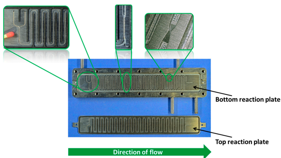
Figure 1. Orifice microreactor, top left zoom: 300 \mu\text{m} caterpillar micromixer for the mixing of the hydroperoxide with the potassium hydroxide, central zoom: 300 \mu\text{m} caterpillar micromixer for acid halide dosage, top right zoom: one of the five Venturi-like orifices.
