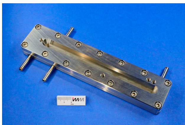
Figure 2. Mounted orifice microreactor, view on the inspection window for infrared measurements.
