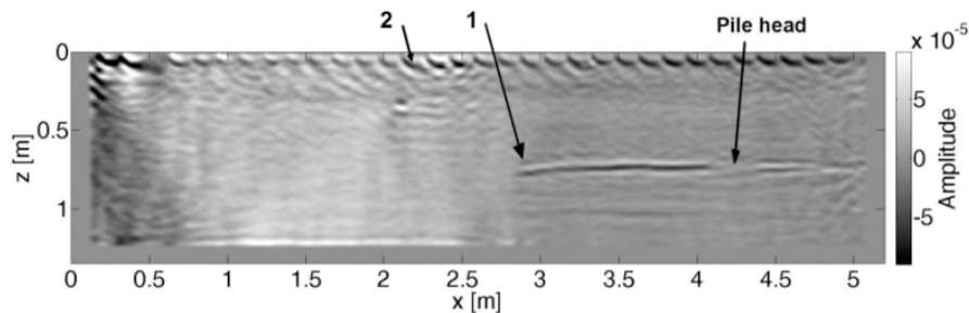
Figure 7. RTM image of the line profile (1: slight dip of the lower boundary of the slab and 2: migration artifacts caused by direct waves)
