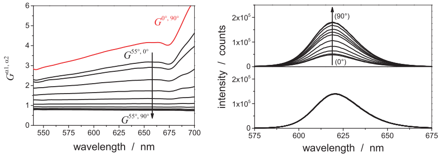
Figure 2: Left: Wavelength dependence of the correction factors G^{\alpha_1, \alpha_2} (see Equation 2) for \alpha_1 = 0^\circ, \alpha_2 = 90^\circ (red) and \alpha_1 = 55^\circ, \alpha_2 = 0^\circ \dots 90^\circ (black) combinations of the emission polarizer (excitation polarizer set to 90^\circ ). Right: Uncorrected ( I_{0^\circ/0^\circ \dots 90^\circ} , top) and corrected ( I_c^{0^\circ \dots 90^\circ} , bottom) emission spectra (see Equation 5) of the QD determined with the emission polarizer set to 0^\circ \dots 90^\circ (excitation polarizer set to 0^\circ ).
