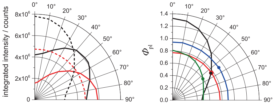
Figure 3: Left: Integrated intensities of uncorrected ( I_c^{55} , solid lines) and corrected ( I_c^{0^\circ \dots 90^\circ} , dotted lines) emission spectra (see Equation 5) of the QD in hexane (red) and RhB in PMMA (black), measured with the excitation polarizer set to 0^\circ in dependence of the angle of the emission polarizer. Right: \Phi_{PL} of the QDR (green) and the QD (red) in hexane, RhB incorporated in PMMA (black), and Rh101 in ethanol (blue) in dependence of the angle of the emission polarizer ( 0^\circ excitation polarizer), using a nearly isotropically emitting reference, i.e., Rh101 in ethanol. Magic angle conditions ( 0^\circ/54.7^\circ ) are indicated by dots (see also Table 1).
