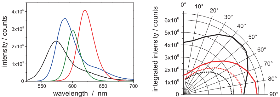
Figure 1: Left: Spectrally corrected emission spectra ( I_c^{55} , \lambda_{\text{ex}} = 530 nm) of the QDR (green) and the QD (red) dispersed in hexane, RhB incorporated in PMMA (black), and Rh101 dissolved in ethanol (blue). Right: Integrated emission intensities obtained from the uncorrected emission spectra with the excitation polarizer set to 0^\circ ( I_{0^\circ/0^\circ\dots90^\circ} , solid lines) and 90^\circ ( I_{90^\circ/90^\circ\dots90^\circ} , dotted lines), respectively, in dependence of the angle of the emission polarizer for the QD in hexane (red) and RhB in PMMA (black).
