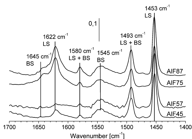
Fig. 4 FTIR spectra of the aluminum hydroxide fluoride samples after stepwise pyridine adsorption and desorption of excess pyridine. The spectra of AIF45 and AIF57 are magnified by a factor of five.
