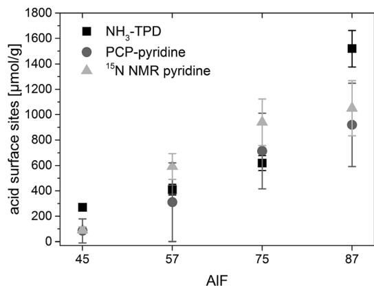
Fig. 2 Concentrations of acidic sites determined by the three methods NH 3 -TPD, PCP-pyridine and 15 N NMR pyridine. Errors shown correspond to standard deviation (STD) of several measurements (NH 3 -TPD), 1.5 STD of several simulations ( 15 N NMR pyridine) or are calculated from linear regression (PCP-pyridine).
