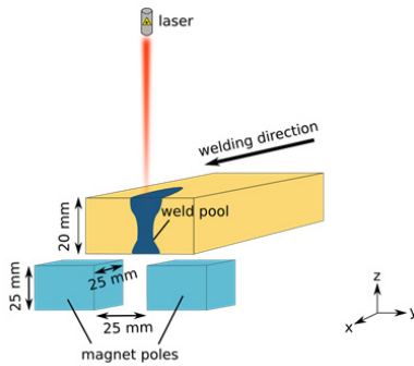
Fig. 4. Setup for the simulation of an electromagnetic weld pool support system.
