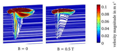
Fig. 10. Velocity streamlines in the weld pool without and with magnetic control for a welding speed of 0.5 m/min.
