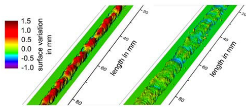
Fig. 15. Weld surface variations for the reference case (left) and case (c) from Figure 14.
