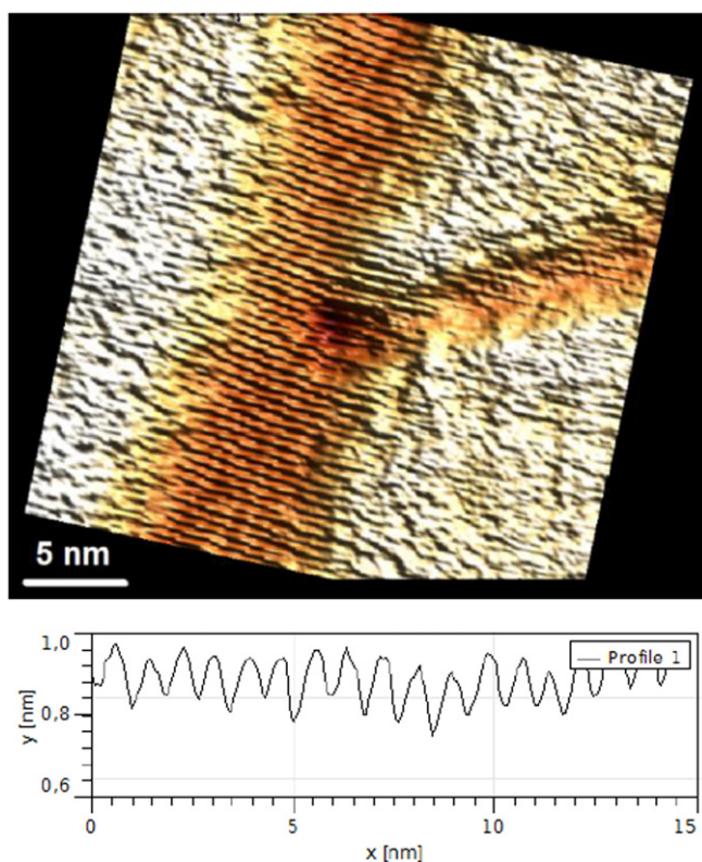
Figure 5. Upper part: STM image of a graphene membrane suspended over a 10 nm wide nanotrench of the Cu(1 1 1) substrate, displaying the characteristic graphene ripples. Lower part: STM line scan showing the magnitude of the ripples. Reproduced with permission from [64]. Copyright 2012 Nature.
