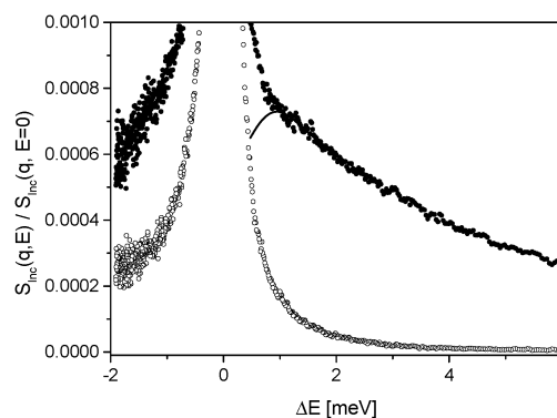
Fig. 9 IN6 spectra of HAT10 normalized to the height of the elastic peak (corresponding to a q range of 1.1 – 2.0 \text{ \AA}^{-1} for elastic scattering): filled circles at T = 80 K; open circles correspond to a measurement at 2 K representing the instrumental resolution. The black solid line is a guide for the eyes. The data were averaged over the detector range 54 – 108^\circ which is the range from which the VDOS was evaluated.
