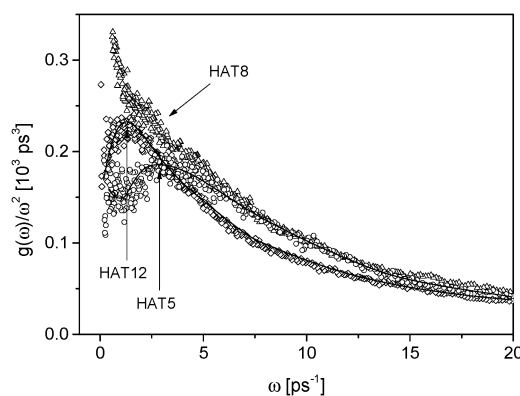
Fig. 14 VDOS of HAT_n with different lengths of the side chains: diamonds – HAT12, triangles – HAT8, circles – HAT5.
