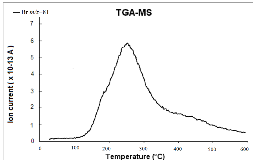
Figure 15. Temperature dependent mass selective ( m/z = 81 ) ion current in TGA-MS analysis of sample CNT1.
