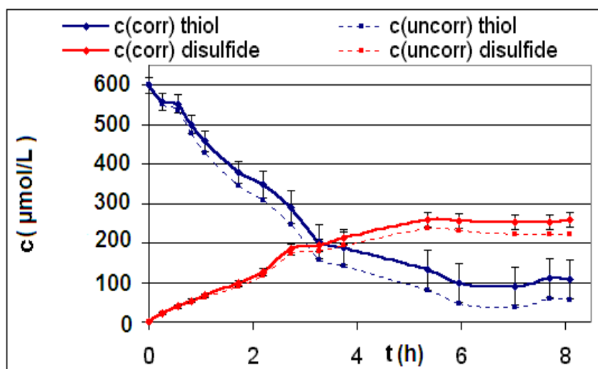
Figure 6. Reaction R6 comparison c_{corr}(t)/c_{uncorr}(t) .
