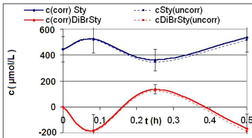
Figure 10. Reaction R3 comparison c_{corr}(t)/c_{uncorr}(t) .
