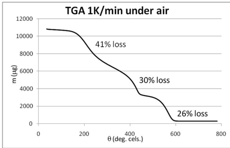
Figure 14. TGA analysis of brominated MWCNT sample CNT1 at 1 K/min under nitrogen.
