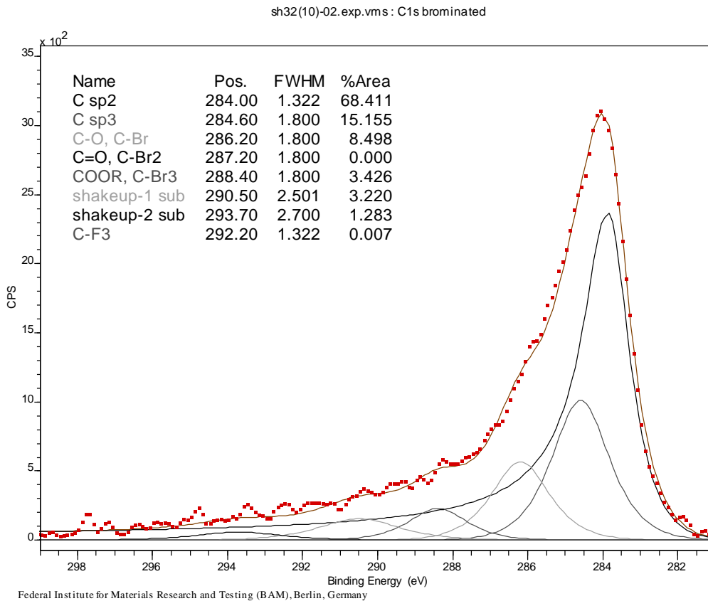
Figure 12. C-1s peak (XPS) of brominated MWCNT sample CNT1.
