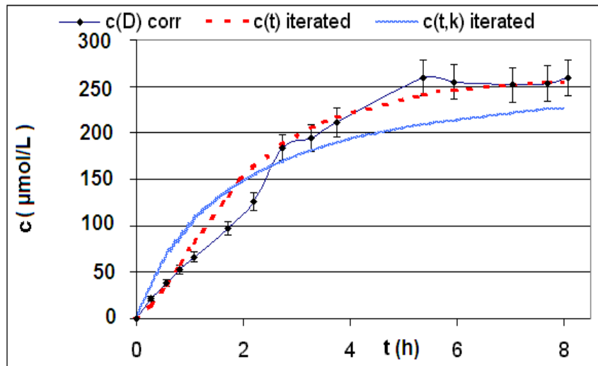
Figure 8. Reaction R1 comparison c_{corr}(t)/C_{uncorr}(t) .
