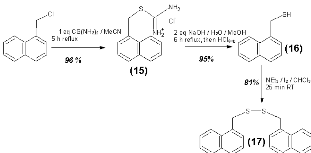
Figure 18. Synthesis steps for substances 15 to 17.
