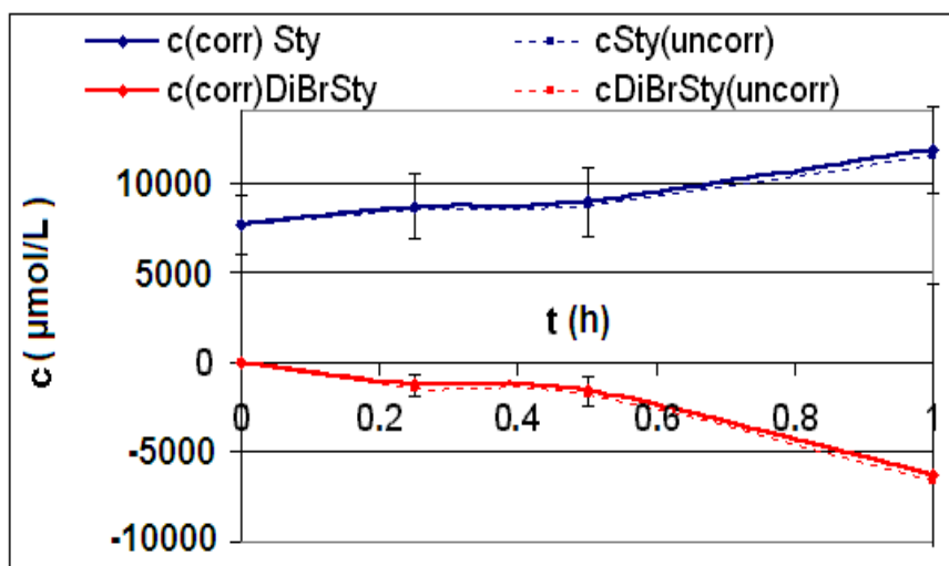
Figure 9. Reaction R2 comparison c_{corr}(t)/C_{uncorr}(t) .
