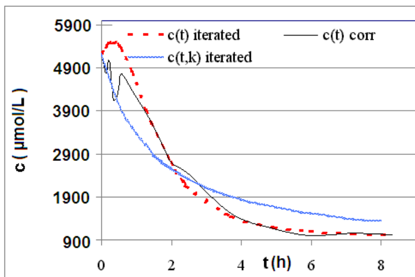
Figure 3. Reaction R4 comparison c_{corr}(t)/c_{iterated}(t)/c_{iterated}(t,k) only for educt thiol A.
