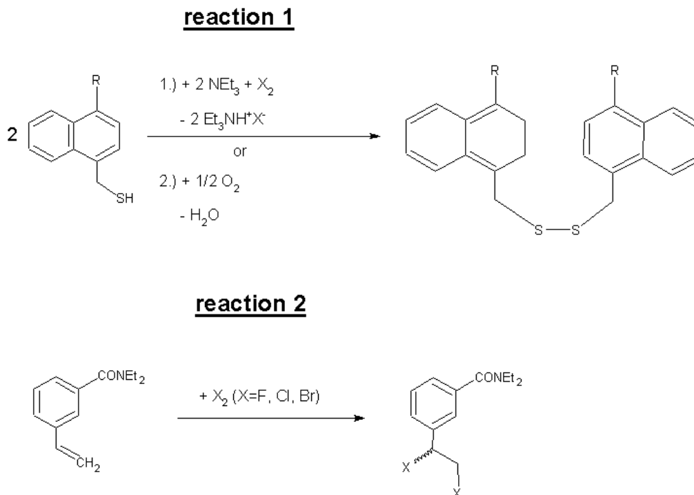
Figure 1. Reactions of substituted (R = organic monovalent rest) 1-naphthylmercaptans with halogens or oxygen and of a substituted 3-styrenecarboxamide with halogens (all at room-temperature (RT)).
