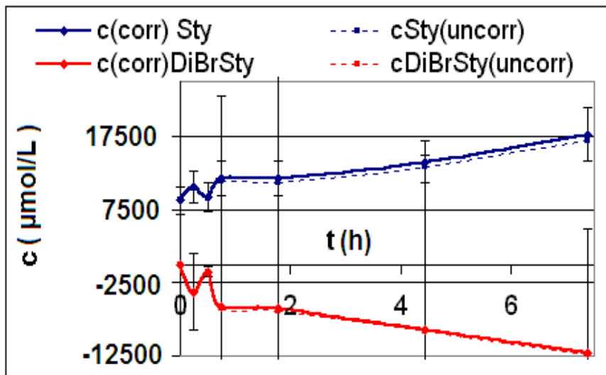
Figure 9. Reaction R2 comparison c_{corr}(t)/C_{uncorr}(t) .
