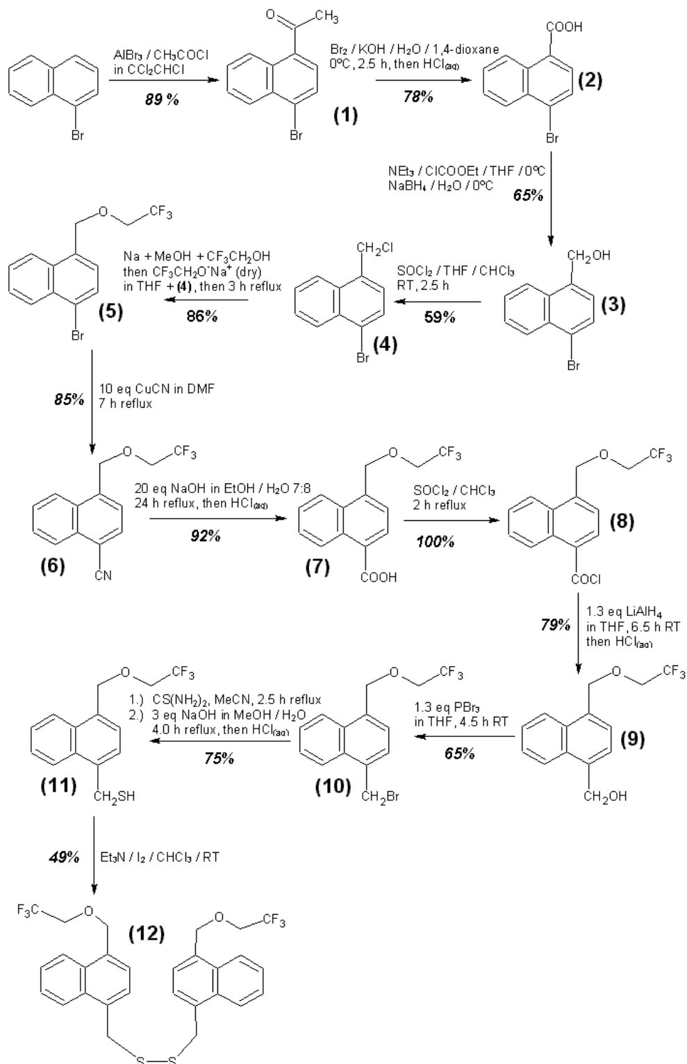
Figure 16. Synthesis steps for substances 1 to 12 .
