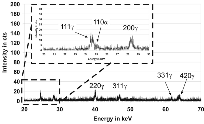
Figure 7. Diffraction pattern at M_s = 195 \text{ }^\circ\text{C} showing martensite and austenite diffractions. Zoomed area represents energy range including first visible martensite diffraction.
