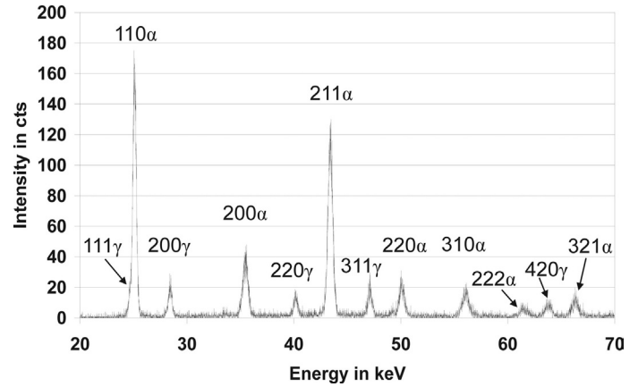
Figure 9. Diffraction pattern at T_d = 35 \text{ }^\circ\text{C} for specimen No. 1 showing martensite and austenite diffractions (martensite formation decays).
