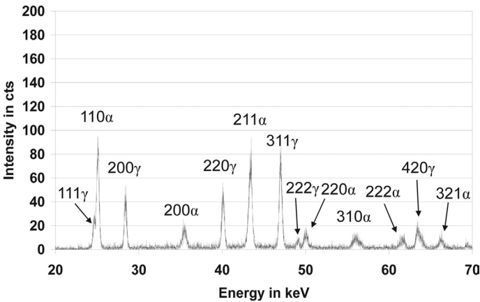
Figure 8. Diffraction pattern at T = 108 \text{ }^\circ\text{C} for specimen No. 1 showing martensite and austenite diffractions.
