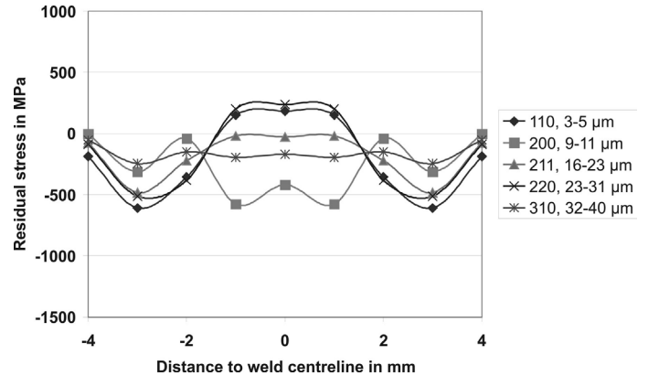
Figure 14. Phase specific longitudinal residual stresses in the martensitic phase of LTT filler No. 1 (8 % Ni, M_s = 184\text{ }^{\circ}\text{C} ) depending on diffraction line and corresponding mean penetration depth \langle\tau\rangle .
