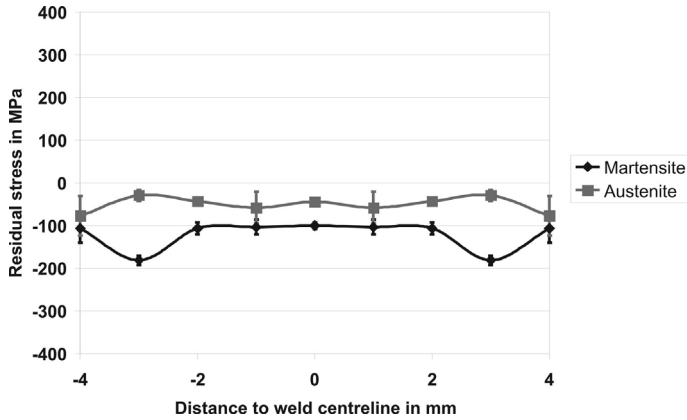
Figure 10. Phase specific longitudinal residual stresses in the martensitic and austenitic phase of LTT filler No. 2 (10 % Ni, M_s = 90\text{ }^{\circ}\text{C} ).
