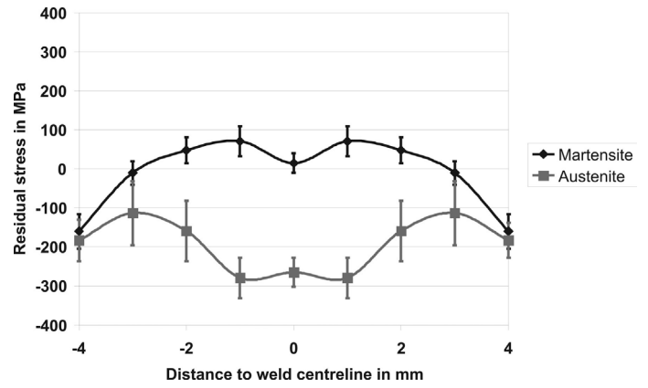
Figure 13. Phase specific transverse residual stresses in the martensitic and austenitic phase of LTT filler No. 3 (12 % Ni, M_s = 39\text{ }^{\circ}\text{C} ).
