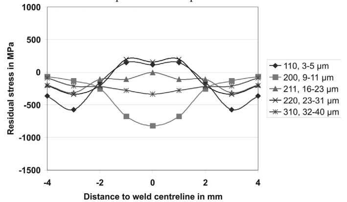
Figure 15. Phase specific longitudinal residual stresses in the martensitic phase of LTT filler No. 2 (10 % Ni, M_s = 90\text{ }^{\circ}\text{C} ) depending on diffraction line and corresponding mean penetration depth \langle\tau\rangle .
