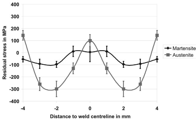
Figure 12. Phase specific longitudinal residual stresses in the martensitic and austenitic phase of LTT filler No. 3 (12 % Ni, M_s = 39\text{ }^{\circ}\text{C} ).
