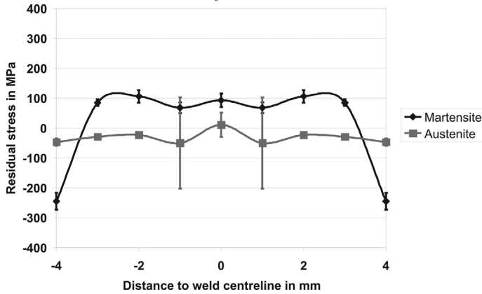
Figure 11. Phase specific transverse residual stresses in the martensitic and austenitic phase of LTT filler No. 2 (10 % Ni, M_s = 90\text{ }^{\circ}\text{C} ).
