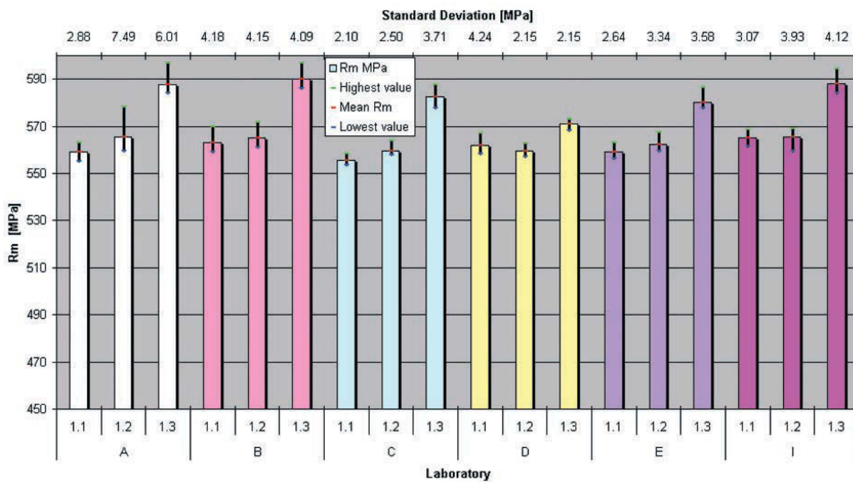
Figure 14 R_m for material 316L with test pieces M16-10 x 50 and extracted outliers
