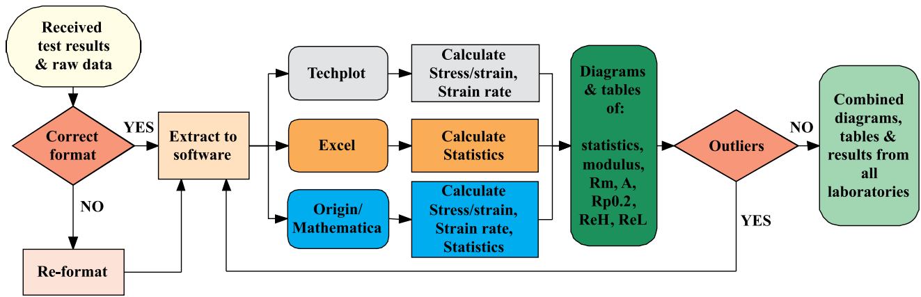
Figure 7 Flow diagram with different steps for data treatment during evaluation of the TENSTAND work package 4 comparison test
