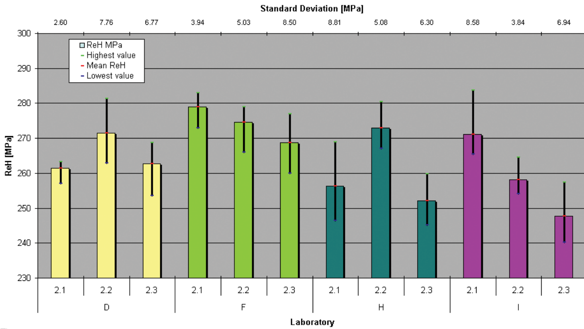
Figure 21 R_{eH} for material ZStE180 with test pieces ISO 12.5 x 50 and extracted outliers
