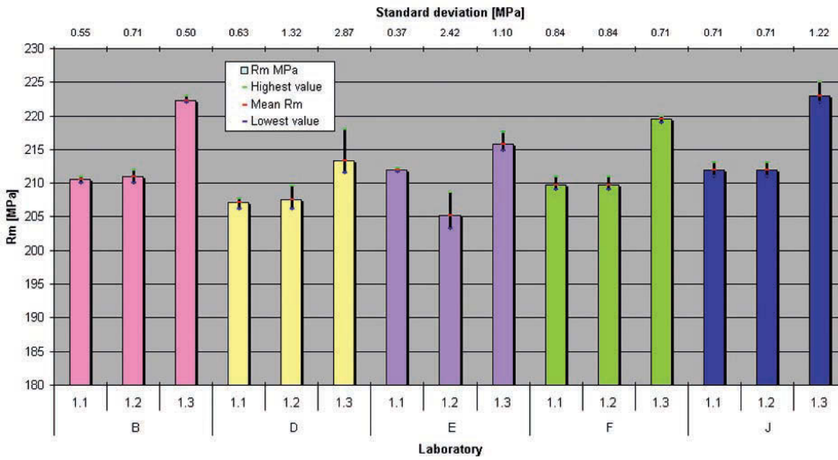
Figure 20 R_m for material AA5754 with test pieces ISO 20 x 80 and extracted outliers
