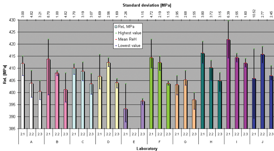
Figure 30 R_{el} for material S355 with test pieces ISO 12.5 x 50 and extracted outliers
