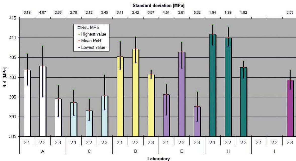
Figure 29 R_{el} for material S355 with test pieces M16-10 x 50 and extracted outliers
