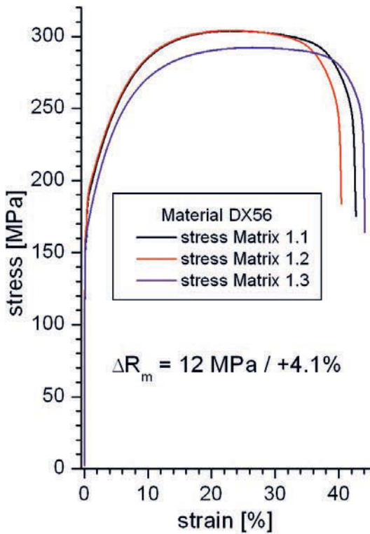
Figure 40 Stress strain curves for modes 1.1, 1.2, and 1.3 at the material DX56
