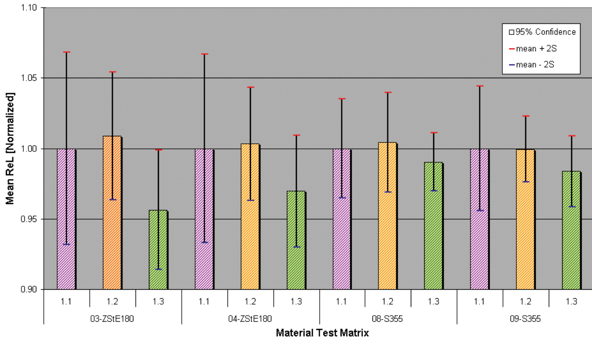
Figure 35 Normalised test results for R_{eL} of the materials ZStE180 and S355
