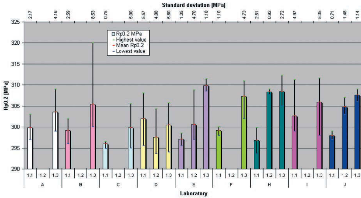
Figure 15 R_{p0.2} for material Nimonic 75 with test pieces M14-10 x 50 and extracted outliers
