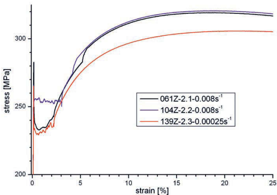
Figure 47 Stress strain curves for ZStE180, mode 2.1, 2.2, 2.3; influence of strain rate on R_m
