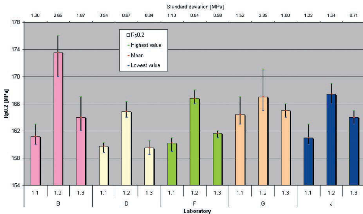
Figure 10 R_{p0.2} for material DX56 with ISO 20 x 80 test pieces and extracted outliers
