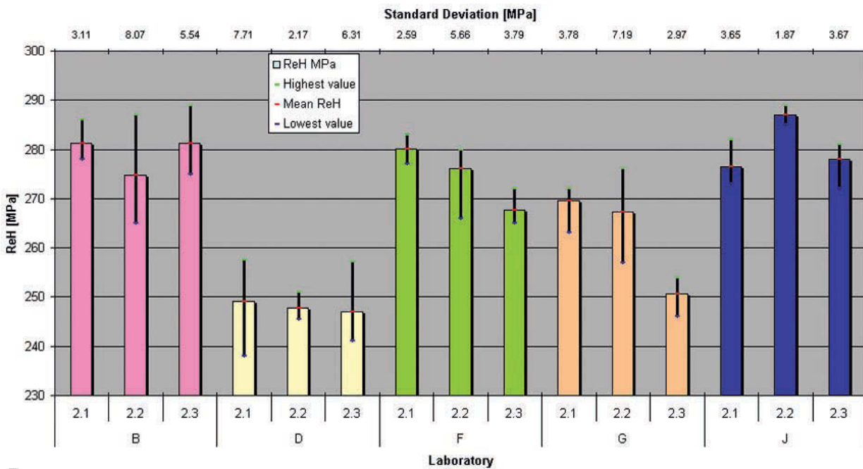
Figure 22 R_{eH} for material ZStE180 with test pieces ISO 20 x 80 and extracted outliers
