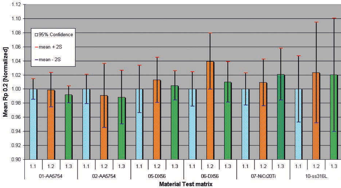
Figure 33 Normalised test results for R_{p0.2} of the materials AA5754, DX56, Nimonic 75 and SS316L
