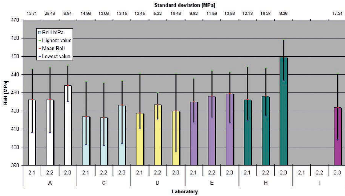
Figure 27 R_{eH} for material S355 with test pieces M16-10 x 50 and extracted outliers
