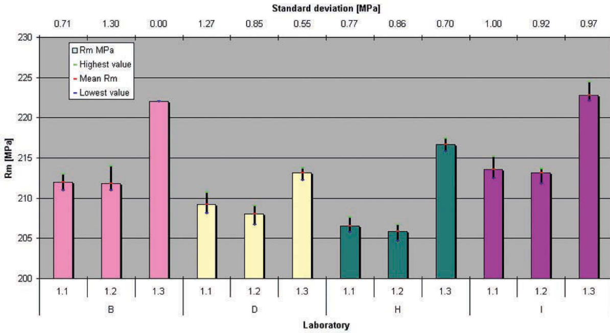
Figure 19 R_m for material AA5754 with test pieces ISO 12.5 x 50 and extracted outliers
