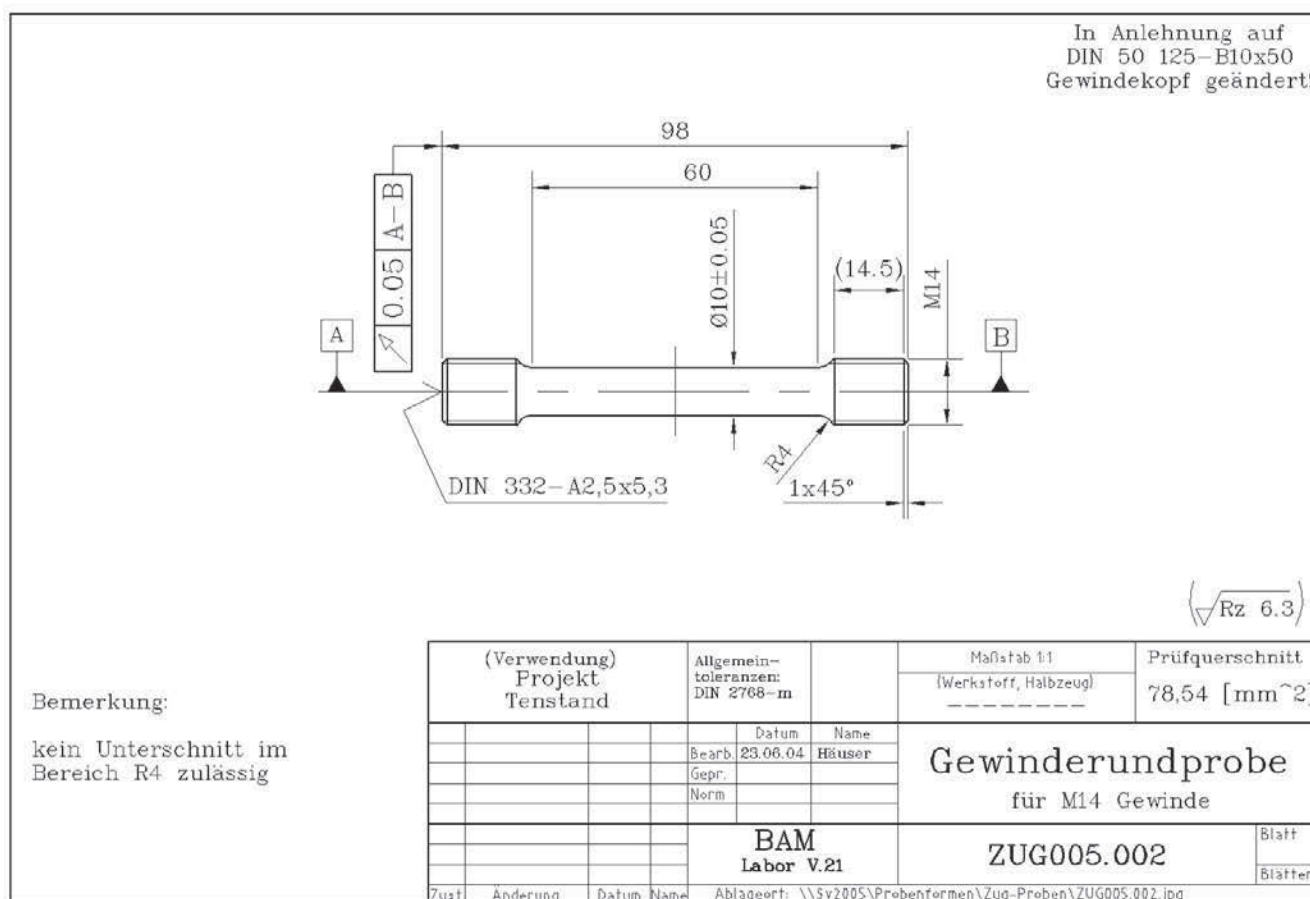
Figure 5 Test piece geometry according to DIN 50125 but with M14 thread for cylindrical threaded samples of Nimonic 75
