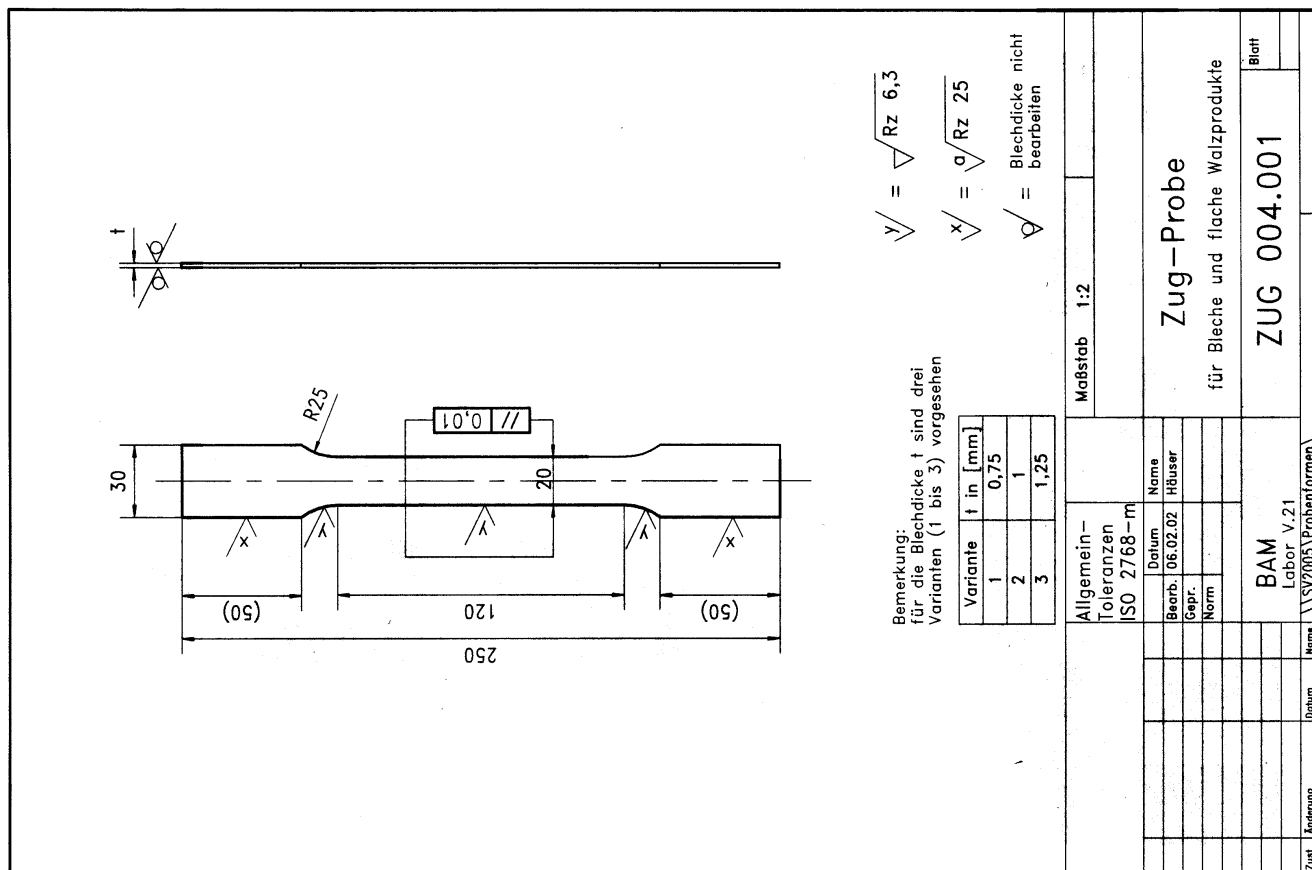
Figure 3 Test piece geometry ISO 20 x 80 for flat samples of the materials AA5754, ZStE180, DX56
