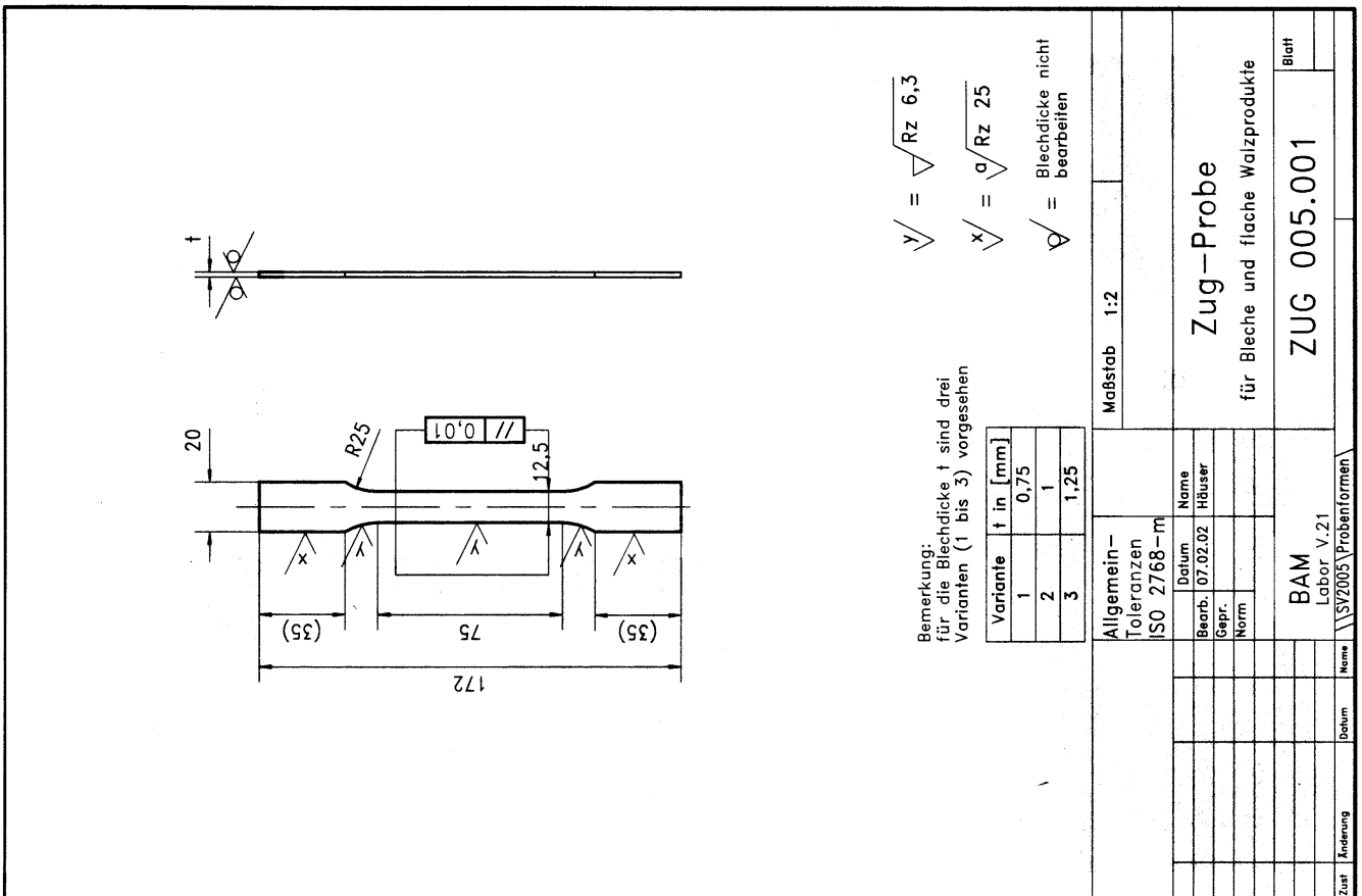
Figure 2 Test piece geometry ISO 12.5 x 50 for flat samples of the materials AA5754, ZStE180, S355
