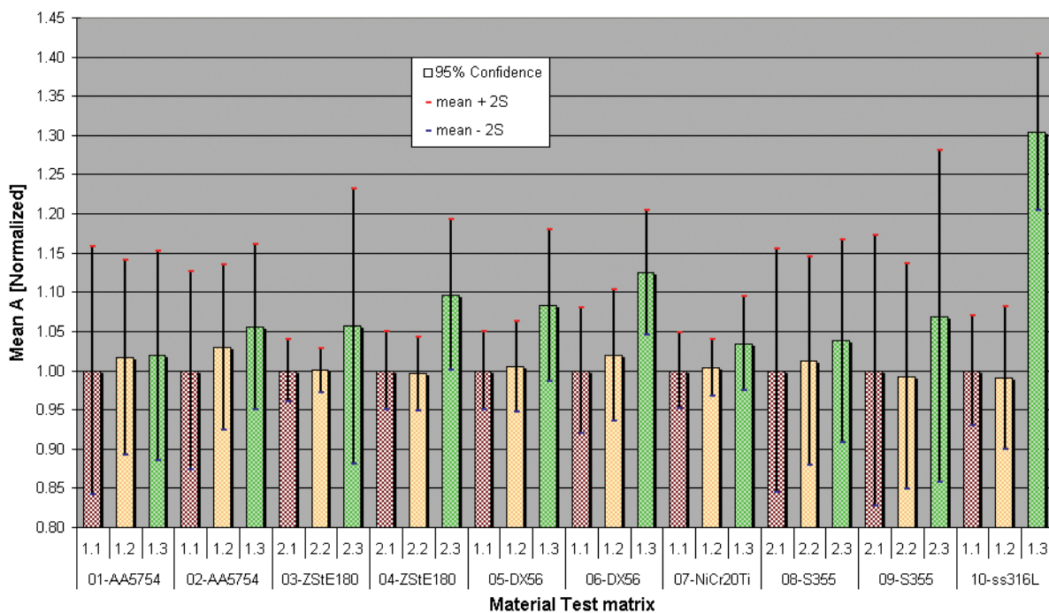
Figure 37 Normalised test results for A of the materials AA5754, ZStE180, DX56, Nimonic 75, S355 and SS316L
