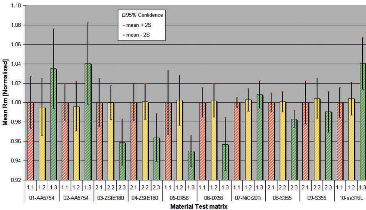
Figure 36 Normalised test results for R_m of the materials AA5754, ZStE180, DX56, Nimonic 75, S355 and SS316L
