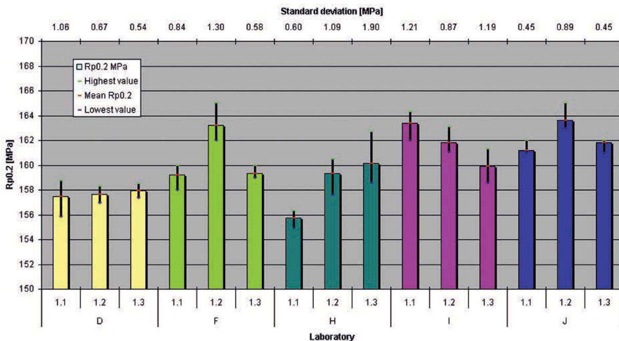
Figure 9 R_{p0.2} for material DX56 with ISO 12.5 x 50 test pieces and extracted outliers
