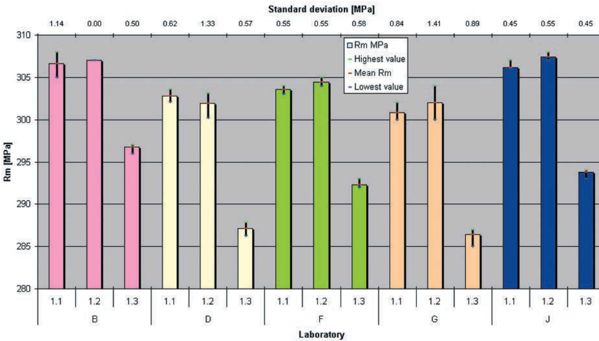
Figure 12 R_m for material DX56 with ISO 20 x 80 test pieces and extracted outliers
