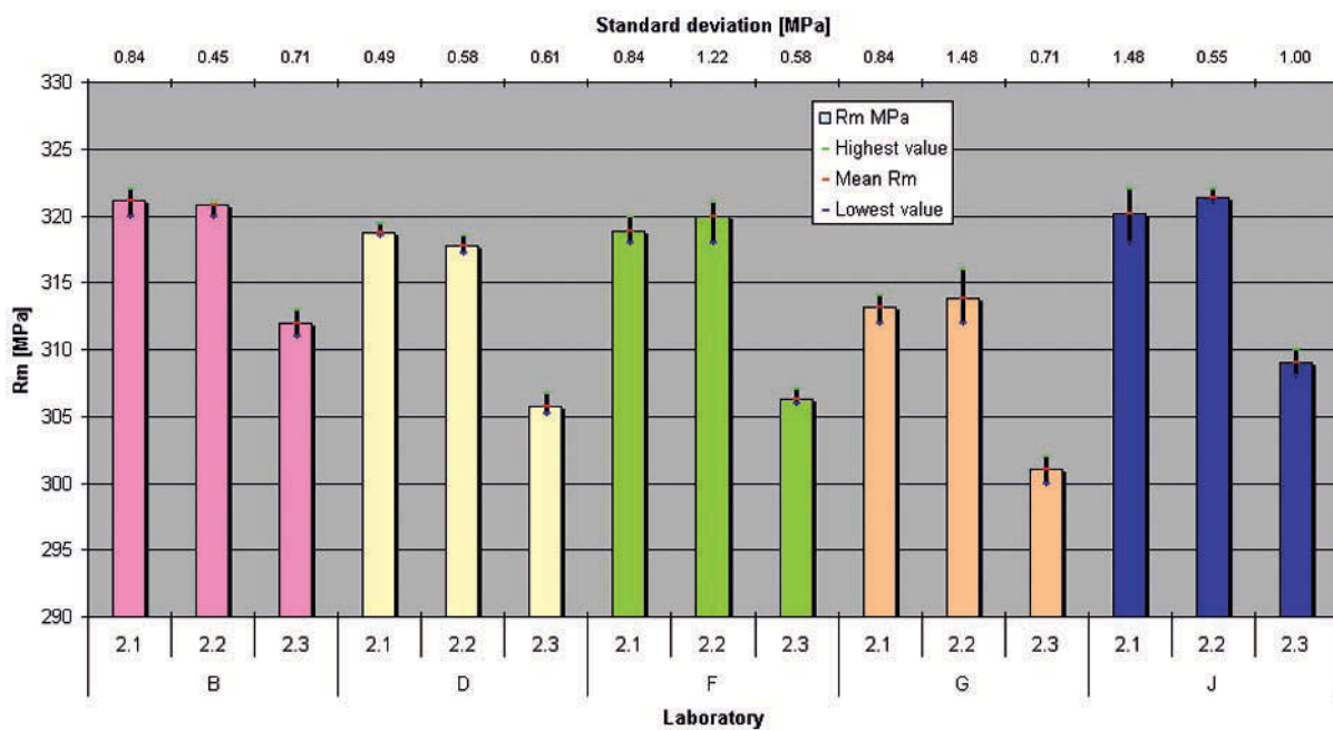
Figure 26 R_m for material ZStE180 with test pieces ISO 20 x 80 and extracted outliers
