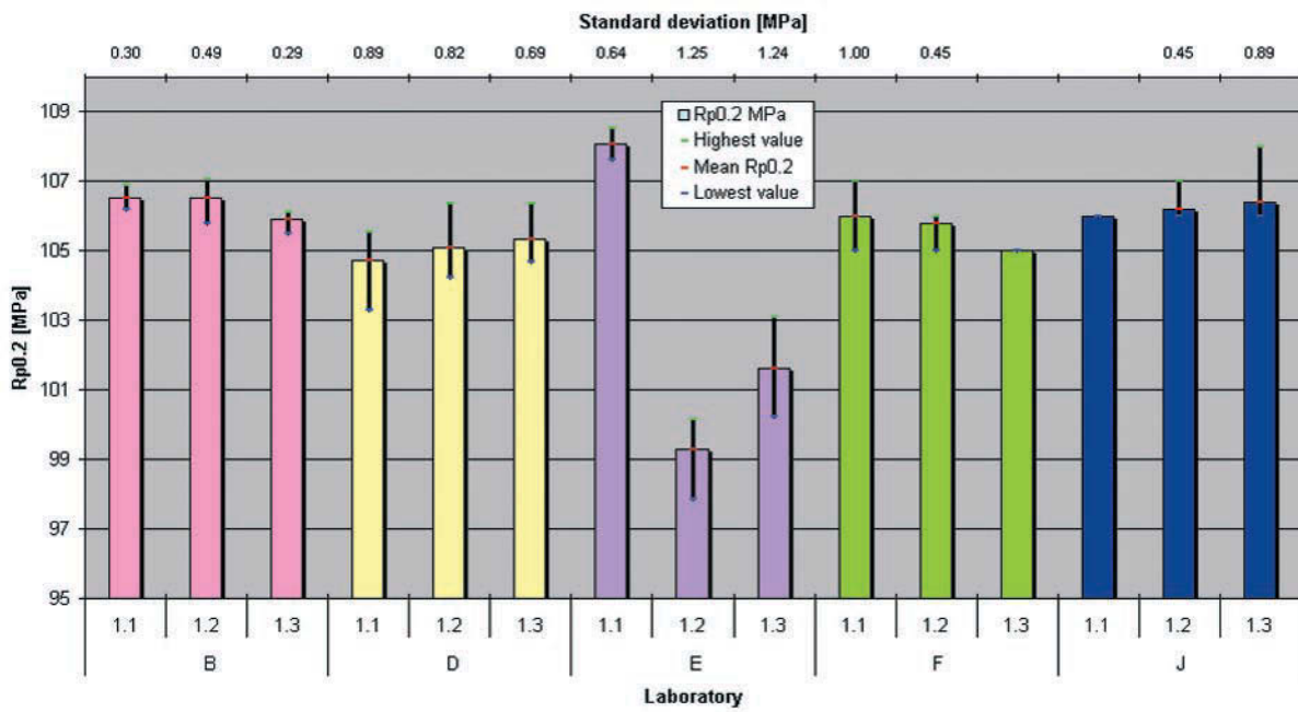
Figure 18 R_{p0.2} for material AA5754 with test pieces ISO 20 x 80 and extracted outliers
