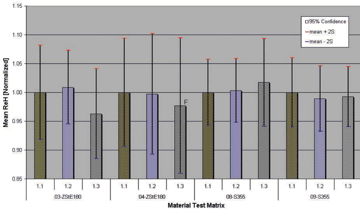
Figure 34 Normalised test results for R_{eH} of the materials ZStE180 and S355
