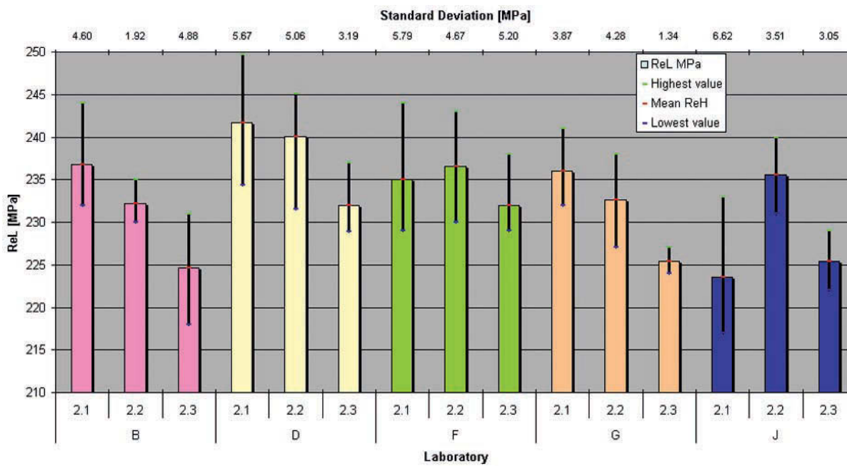
Figure 24 R_{eL} for material ZStE180 with test pieces ISO 20 x 80 and extracted outliers
