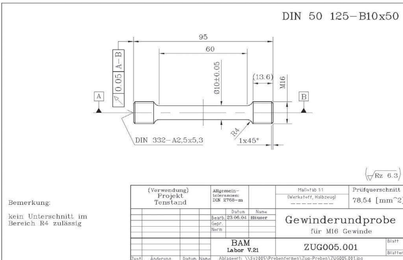
Figure 4 Test piece geometry according to DIN 50125 for cylindrical threaded samples of S355 and 316L
