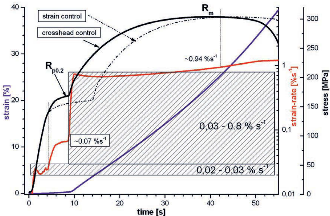
Figure 41 Stress, strain and strain rate vs. time for DX56 (ISO 20 x 80) for modes 1.1 and 1.2 and the allowed testing speed
