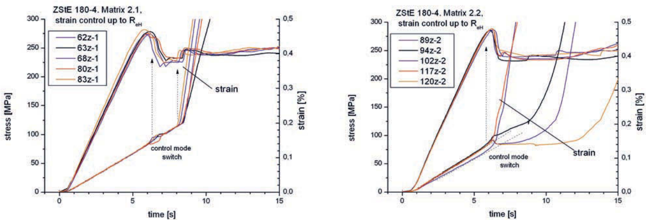
Figure 43 Stress, strain vs. time for ZStE180, mode 2.1 and 2.2
