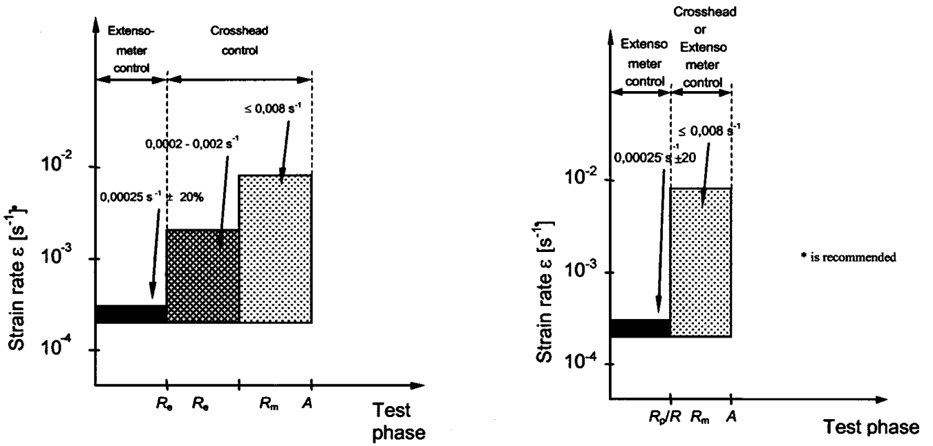
Figure 1 Proposal of ECISS TC1 WG1 to determine the allowed testing speeds for initially strain controlled tensile testing
