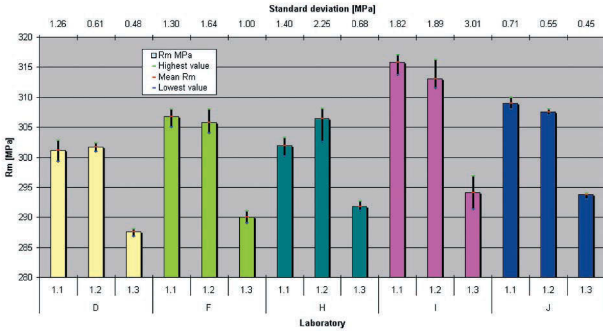
Figure 11 R_m for material DX56 with ISO 12.5 x 50 test pieces and extracted outliers
