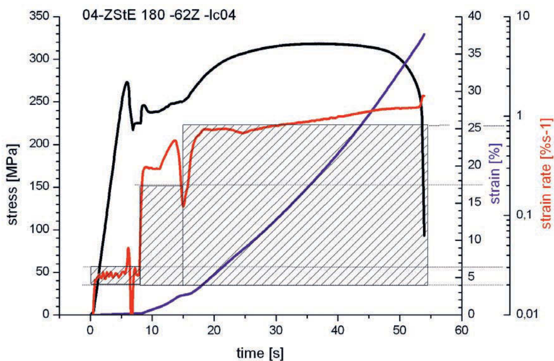
Figure 46 Stress, strain, strain rate for ZStE180, mode 2.1, allowed testing speed
