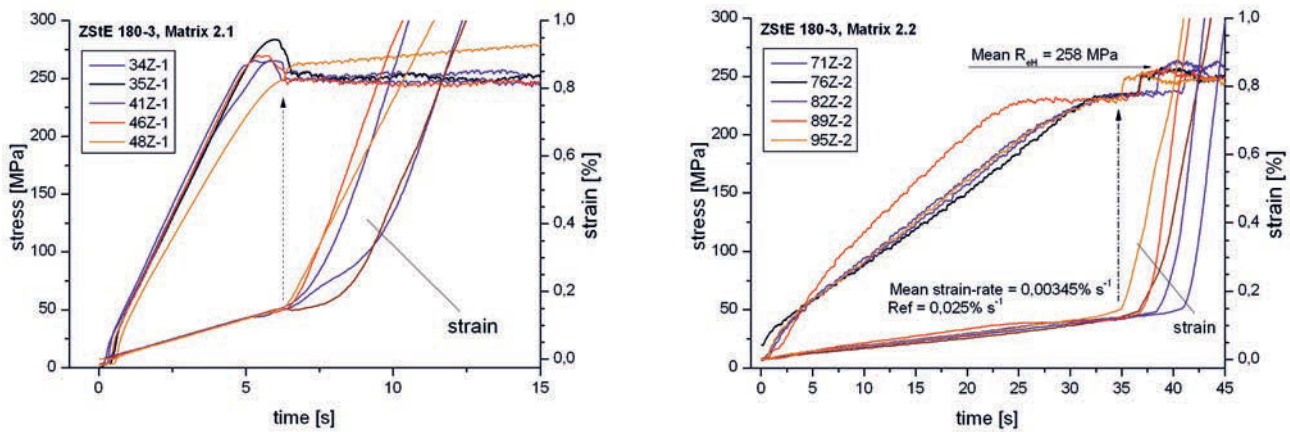
Figure 44 Stress, strain vs. time for ZStE180, mode 2.1 and 2.2
