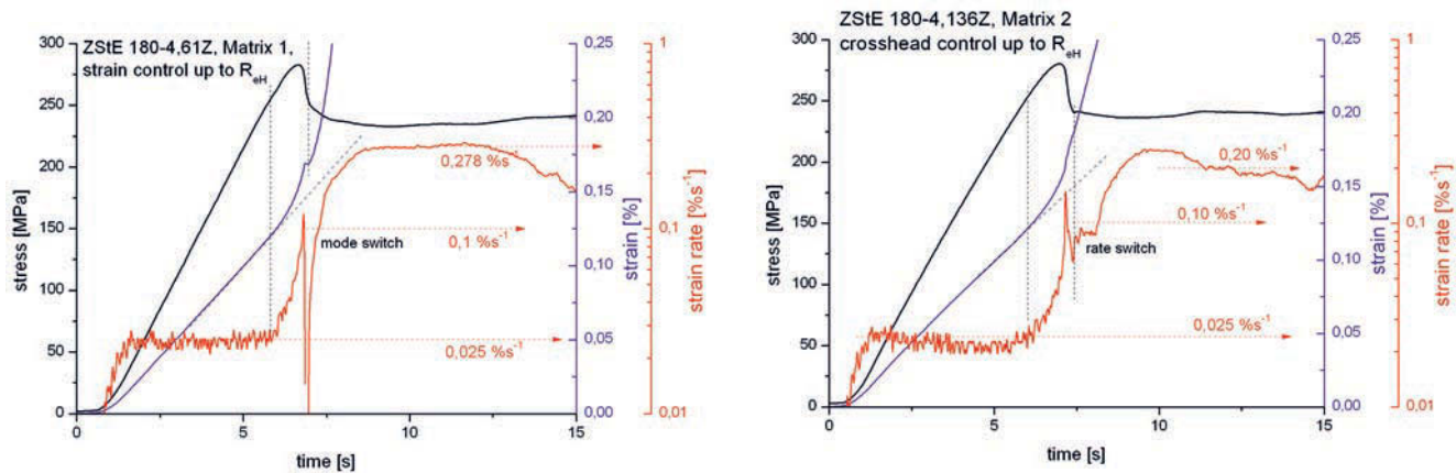
Figure 45 Stress, strain, strain rate vs. time for ZStE180, mode 2.1 and 2.2
