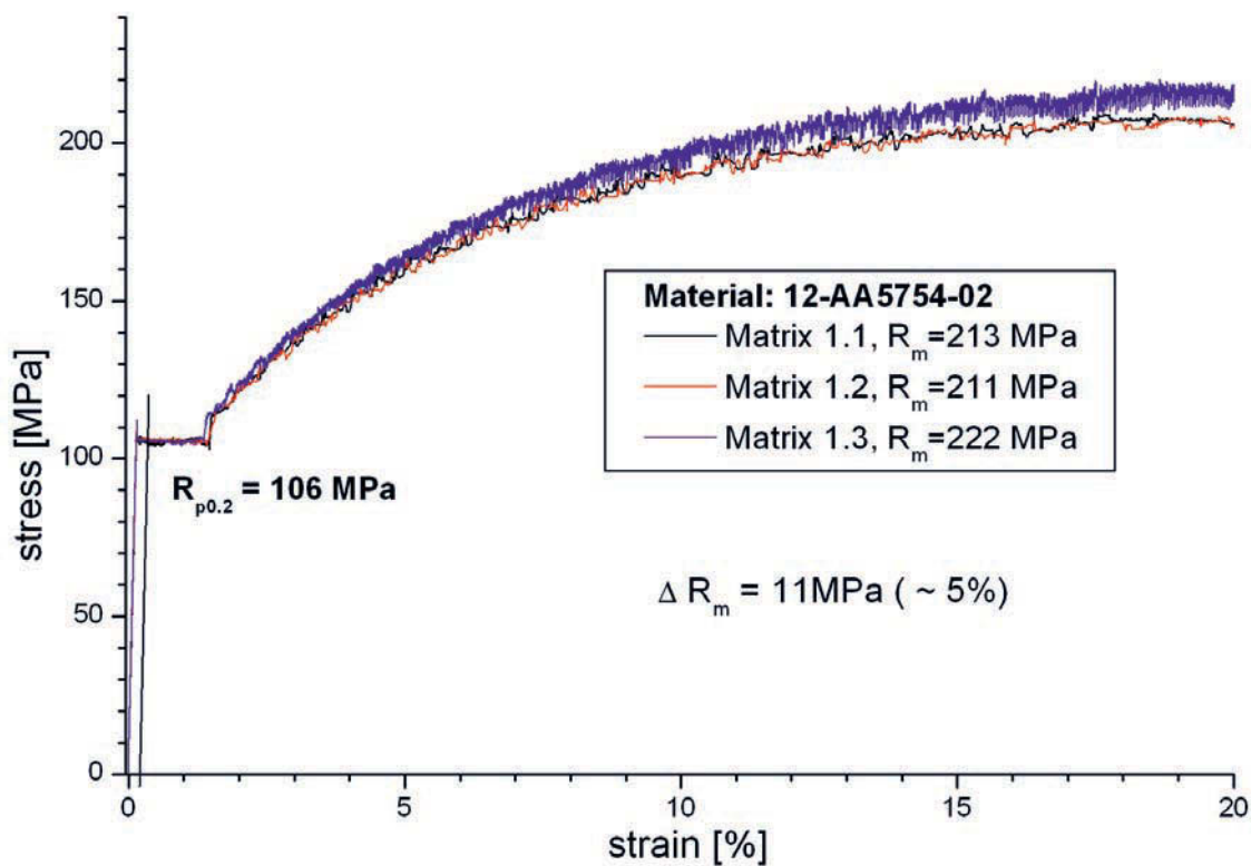
Figure 42 Stress strain curves for AA5754 (ISO 20 x 80) for modes 1.1, 1.2 and 1.3
