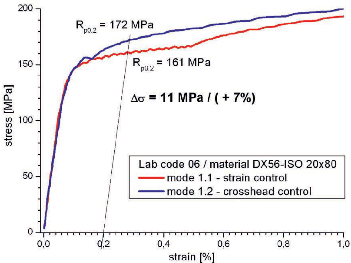
Figure 38 Stress strain curves until 1% strain for material DX56 with different values for R_{p0.2} for different control modes
