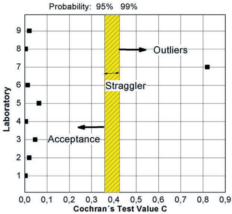
Figure 8 Cochran test for the determination of an outlier
