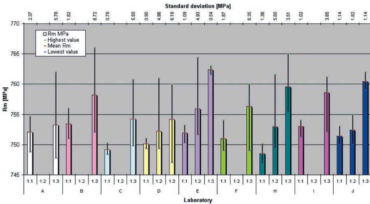
Figure 16 R_m for material Nimonic 75 with test pieces M14-10 x 50 and extracted outliers
