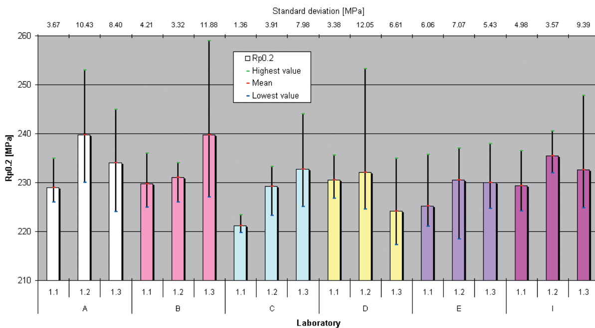
Figure 13 R_{p0.2} for material 316L with test pieces M16-10 x 50 and extracted outliers
