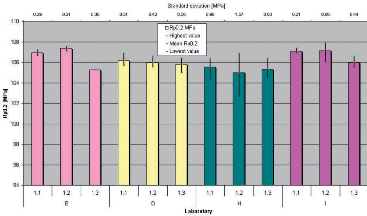
Figure 17 R_{p0.2} for material AA5754 with test pieces ISO 12.5 x 50 and extracted outliers
