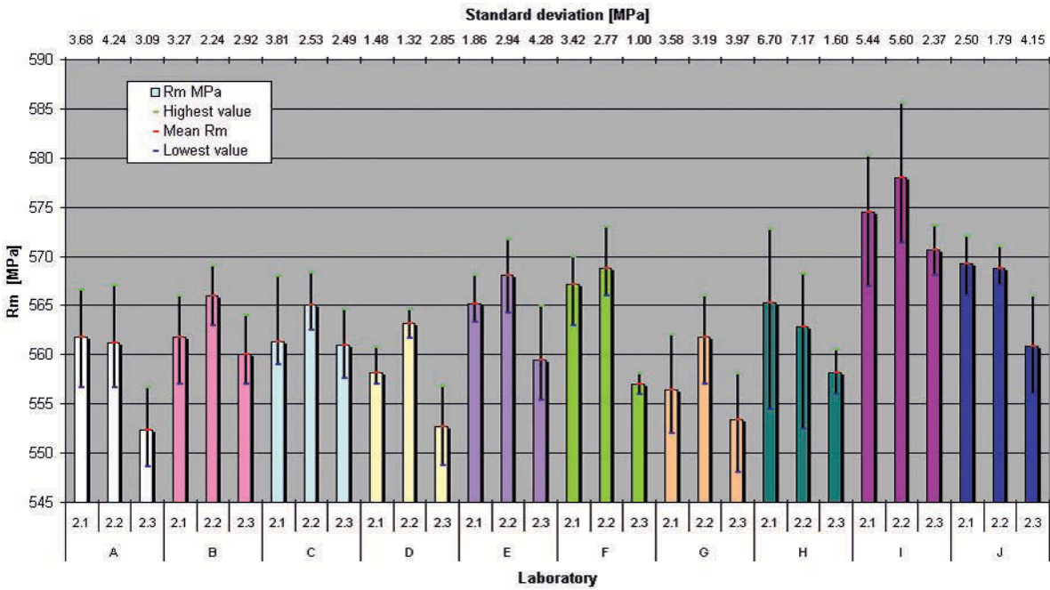
Figure 32 R_m for material S355 with test pieces ISO 12.5 x 50 and extracted outliers
