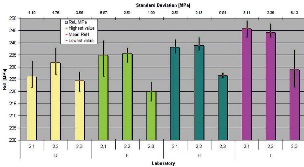
Figure 23 R_{eL} for material ZStE180 with test pieces ISO 12.5 x 50 and extracted outliers
