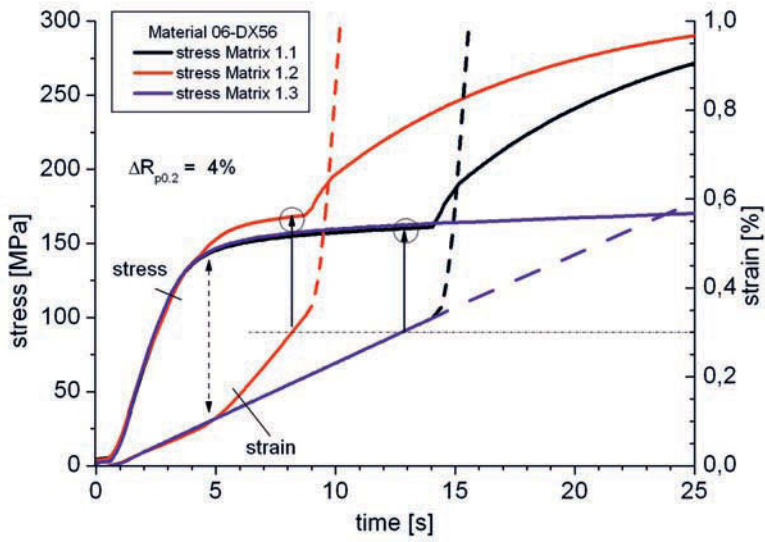
Figure 39 Stress and strain vs. time for the material DX56 (ISO 20 x 80) showing the influence of the control mode and testing speed on R_{p0.2}
