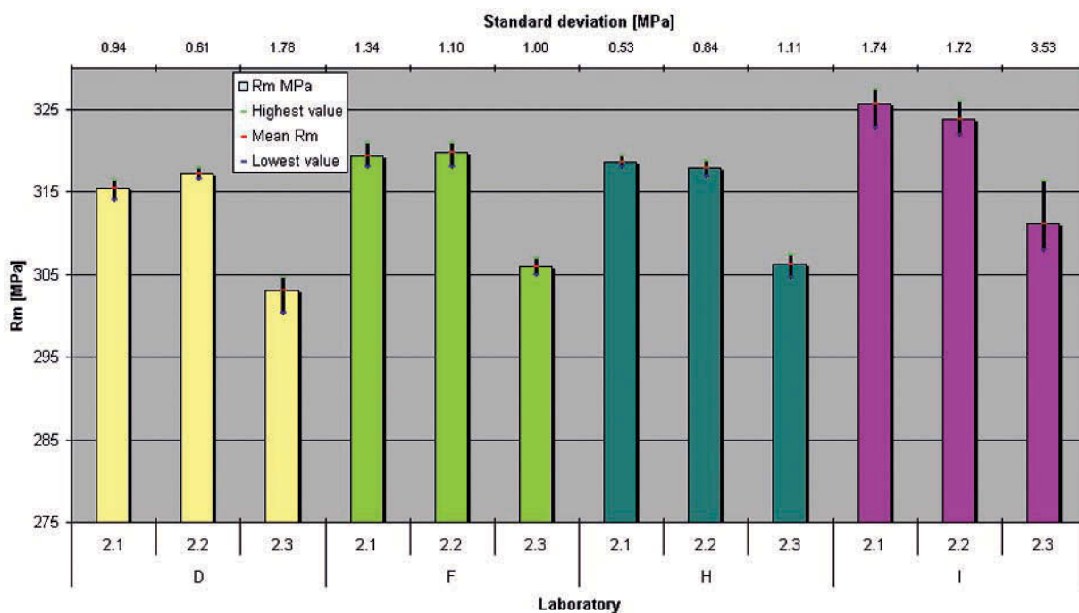
Figure 25 R_m for material ZStE180 with test pieces ISO 12.5 x 50 and extracted outliers
