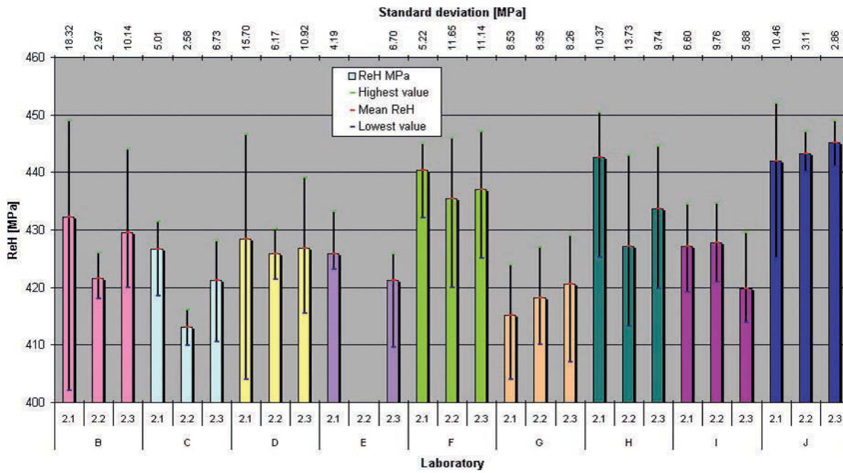
Figure 28 R_{eH} for material S355 with test pieces ISO12.5 x 50 and extracted outliers
