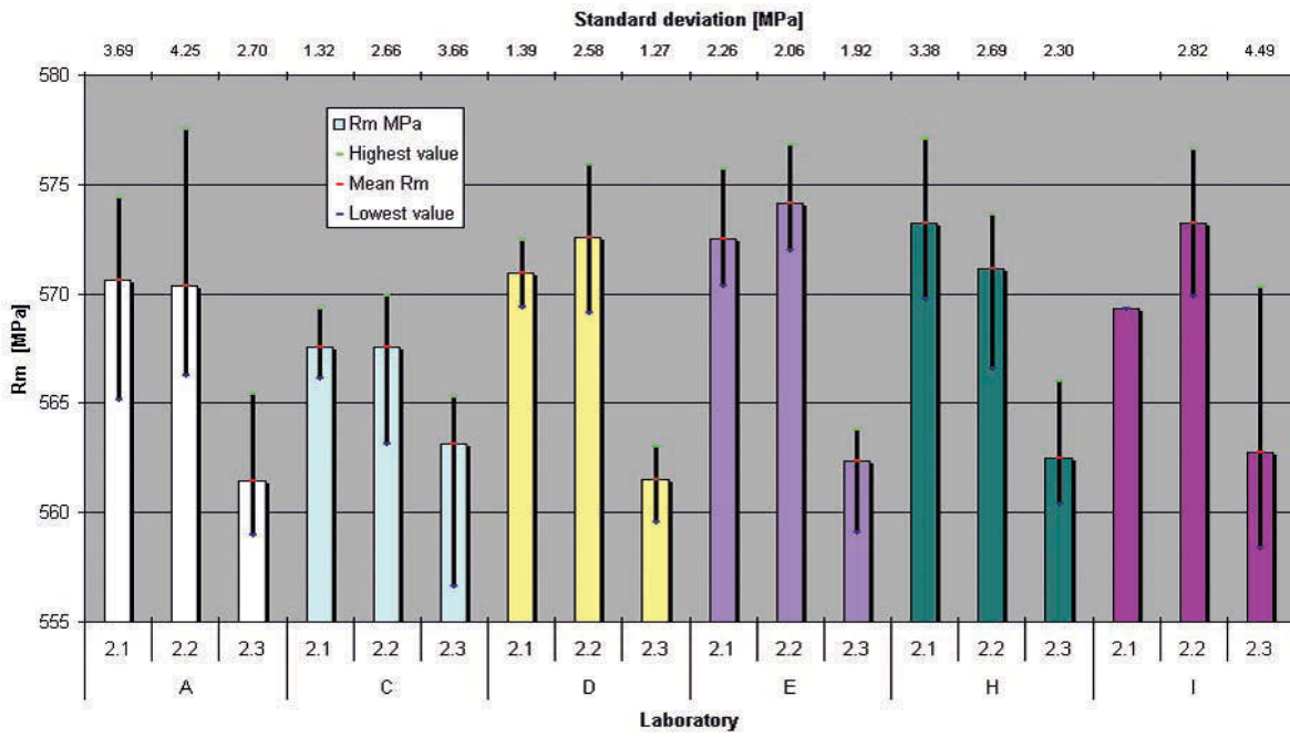
Figure 31 R_m for material S355 with test pieces M16-10 x 50 and extracted outliers
