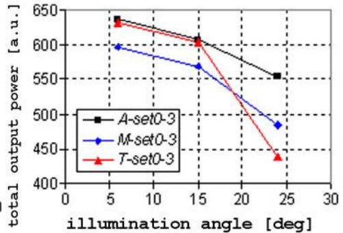
Fig. 6.5 Influence of the illumination angle ( 6^\circ ; 15^\circ ; 24^\circ ) on the total output power of 10 m non-aged fibres.
