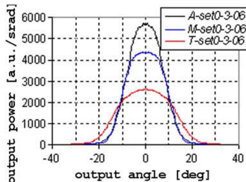
Fig. 6.6 The FFPs of 10 m non-aged fibres from three manufacturers illuminated under 6^\circ angle.
