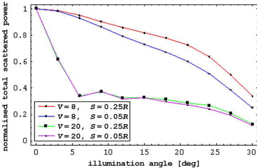
Fig. A2.17 Normalised total scattered power in dependence on the illumination angle.
