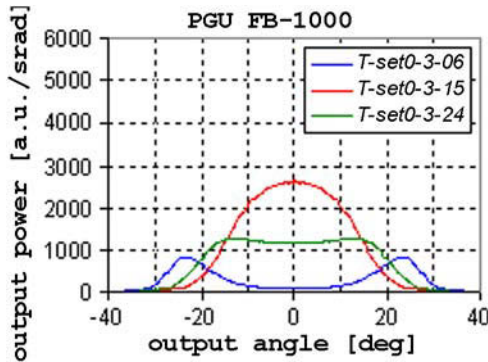
Fig. 6.4 Influence of the illumination angle ( 6^\circ ; 15^\circ ; 24^\circ ) on the FFP of 10 m non-aged Toray's fibre.
