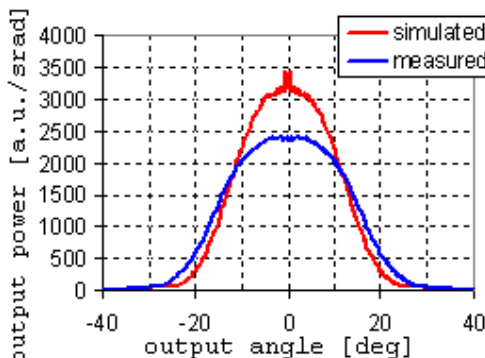
Fig. A3.9 Measured and simulated M-set5-2-06.
