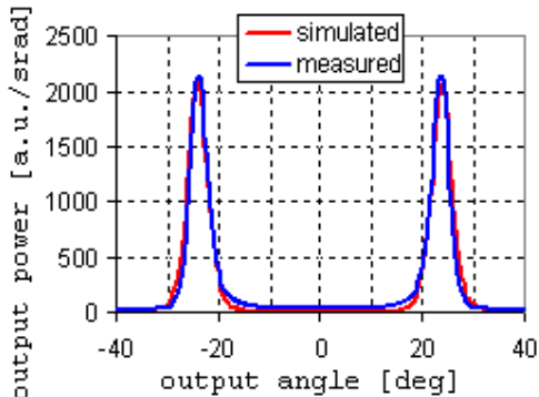
Fig. A3.7 Measured and simulated M-set0-3-24.
