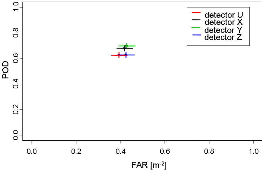
Figure 8.1: Oberjetttenberg May 2003, an ROC diagram for the complete data set, a comparison of detectors. The crosses indicate 95% confidence limits.
