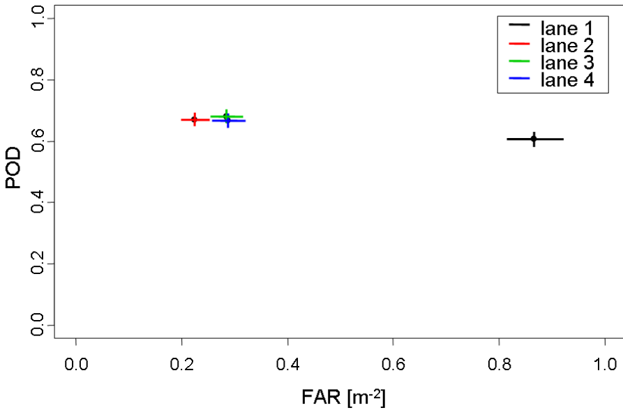
Figure 8.2: Oberjetttenberg May 2003, an ROC diagram for the complete data set, a comparison of lanes. The crosses indicate 95% confidence limits.
